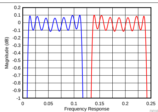
Figure 63. Decimate-by-4 Filter Response (Zoomed)
