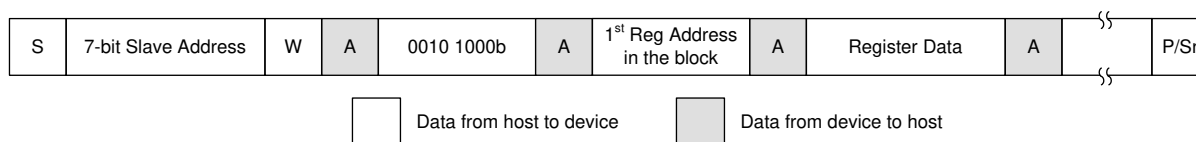
图 8-20. Writing a Continuous Block of Registers
