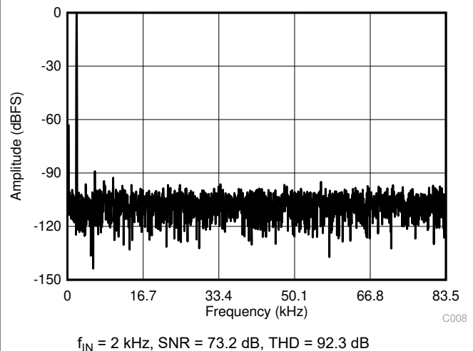
图 7-13. Typical FFT
