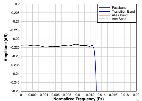
图 8-34. Decimation by 32 complex passband ripple response
