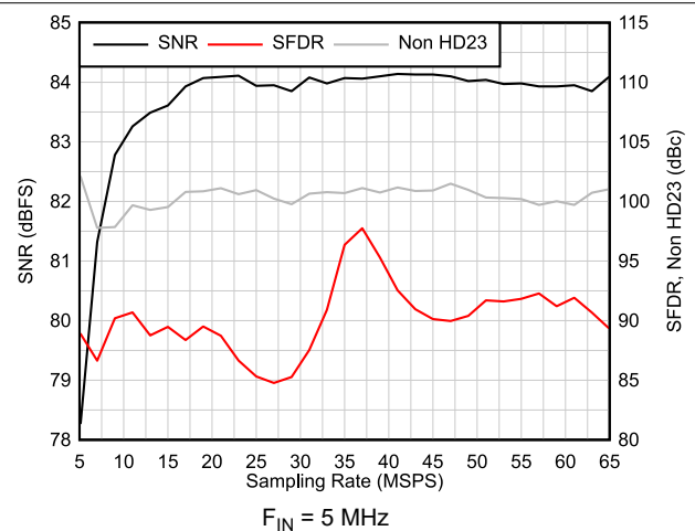
图 6-14. AC Performance vs Sampling Rate
