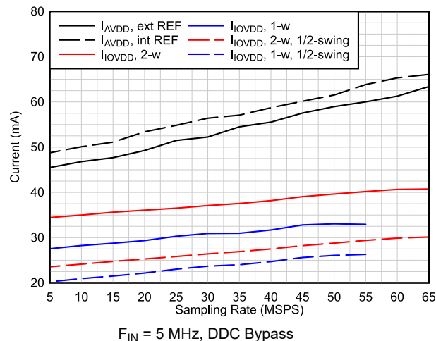
图 6-25. Current vs Sampling Rate
