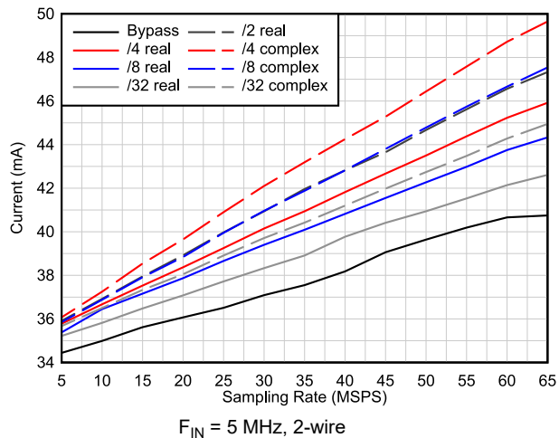
图 6-26. I_{OVDD} Current vs Decimation
