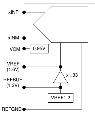
图 8-15. Different voltage reference options for ADC368x
