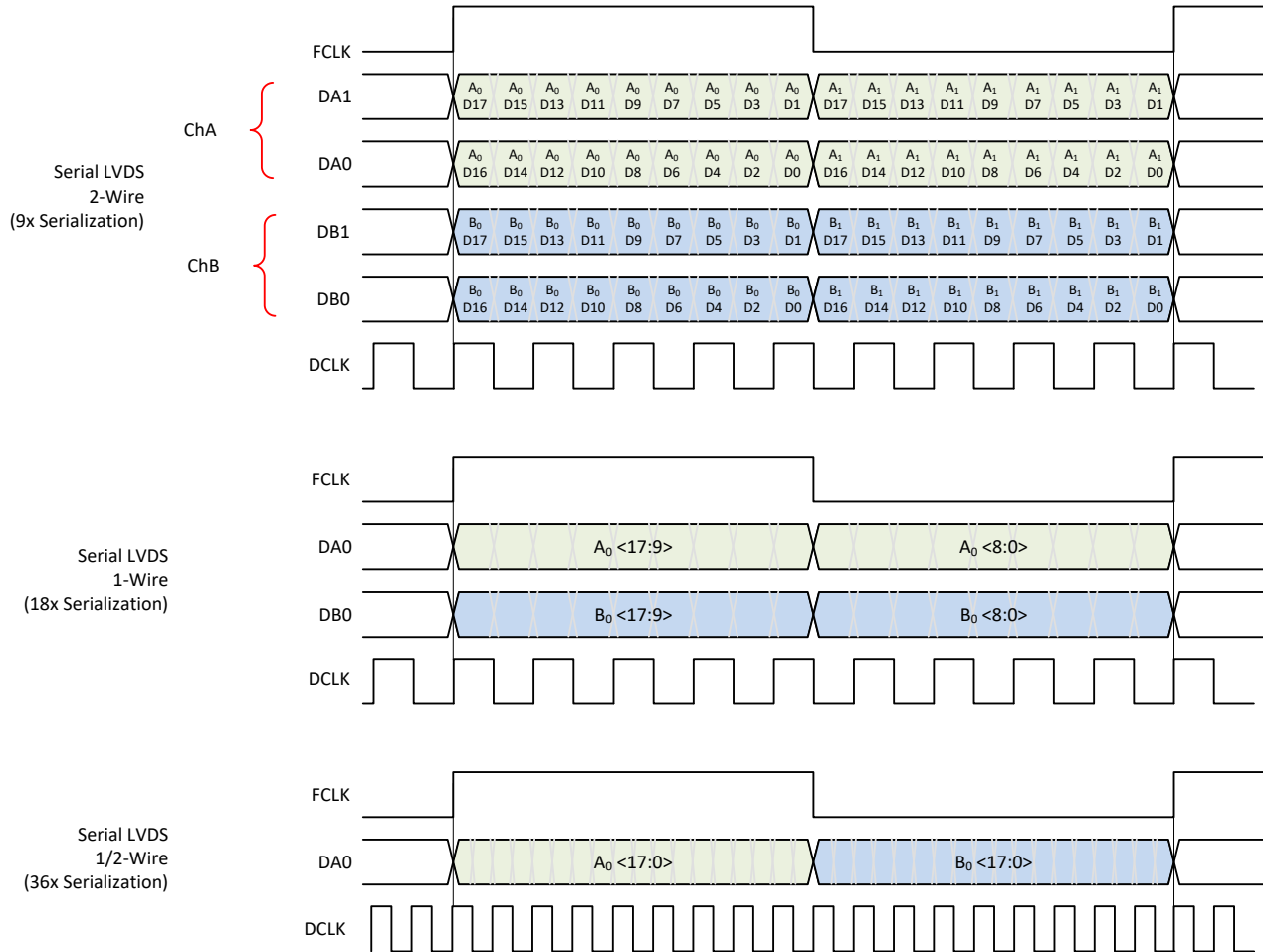
图 8-37. Output Data Format in Real Decimation (18-bit Output Resolution)
