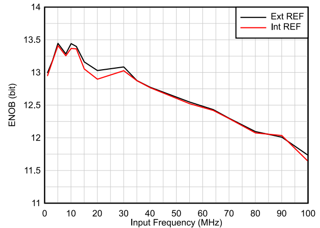
图 6-12. ENOB vs Input Frequency
