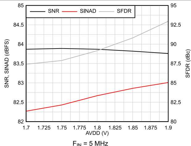
图 6-17. AC Performance vs AVDD
