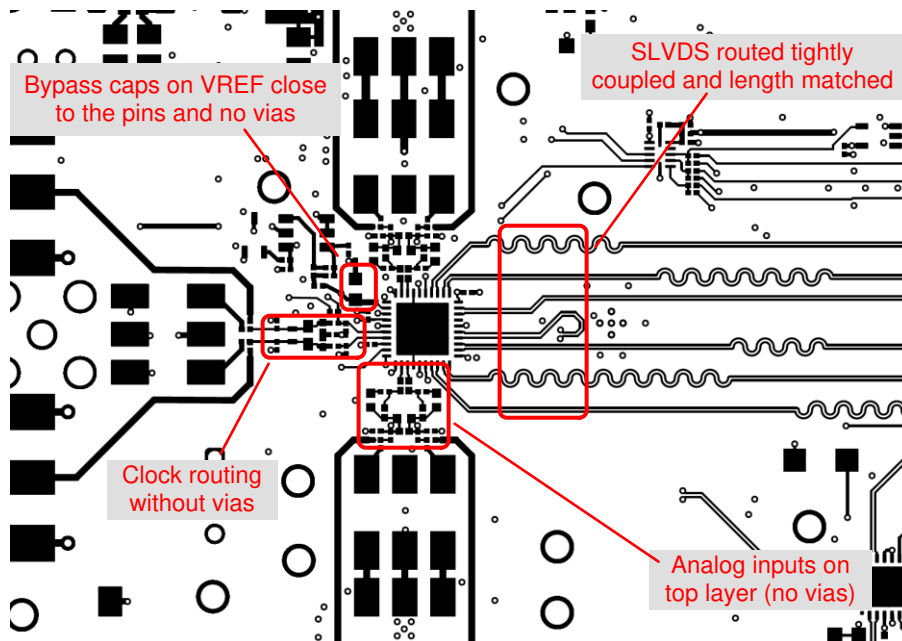
图 11-1. Layout example: top layer of ADC368x EVM
