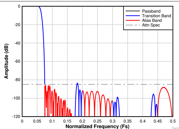
图 8-29. Decimation by 8 complex frequency response
