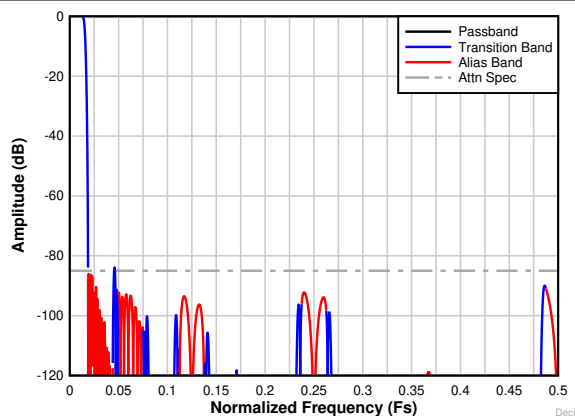
图 8-33. Decimation by 32 complex frequency response
