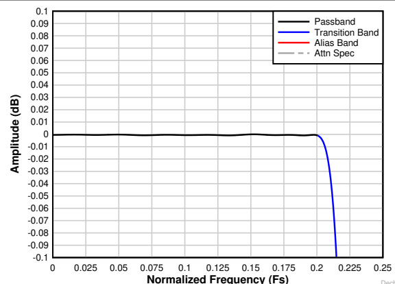
图 8-26. Decimation by 2 complex passband ripple response
