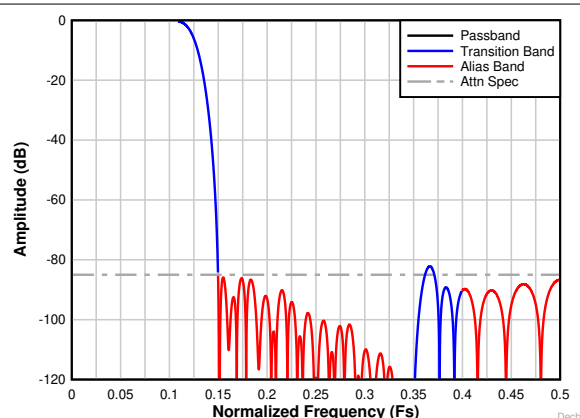
图 8-27. Decimation by 4 complex frequency response
