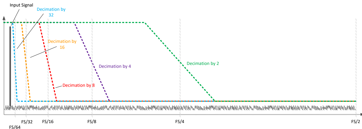
图 8-22. Real decimation illustration
