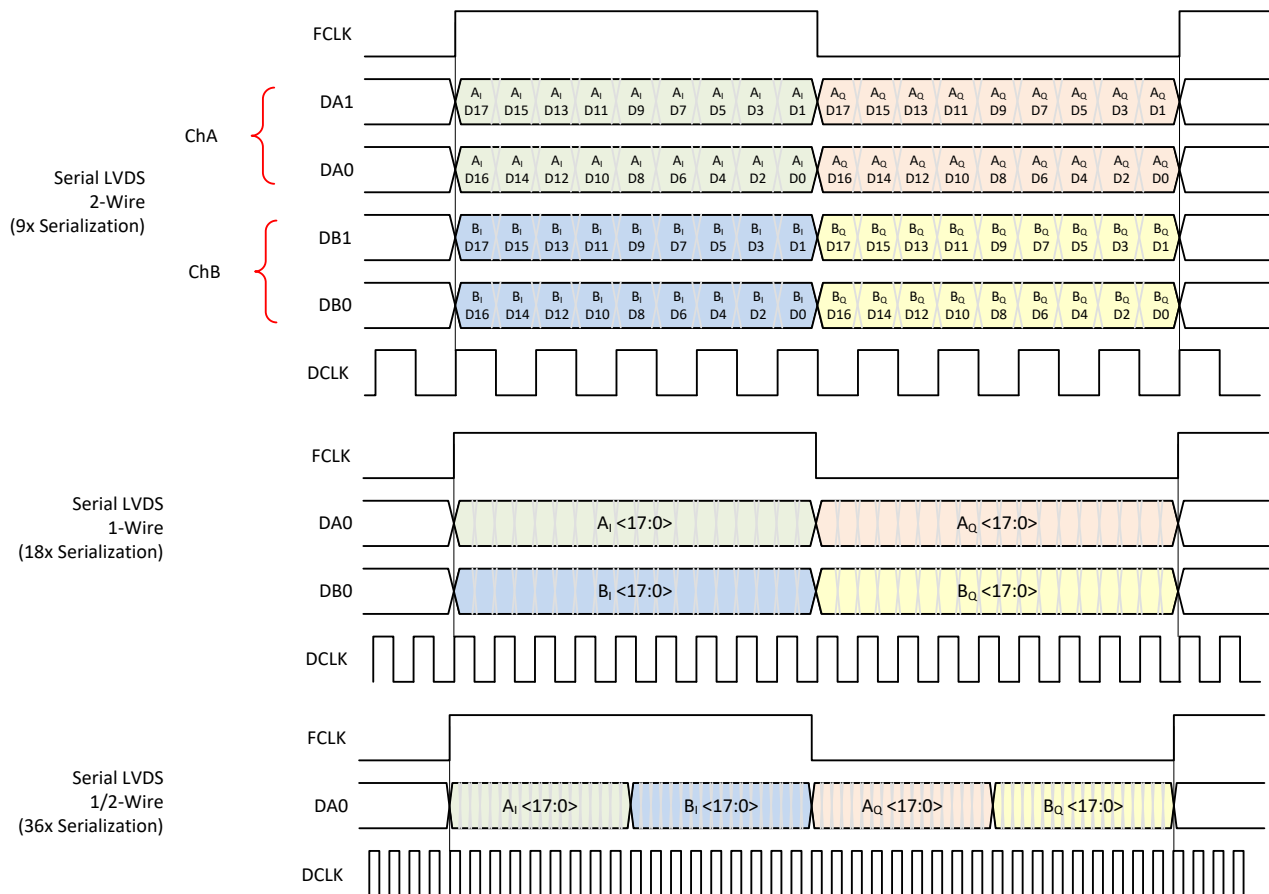
图 8-36. Output Data Format in Complex Decimation (18-bit Output Resolution)
