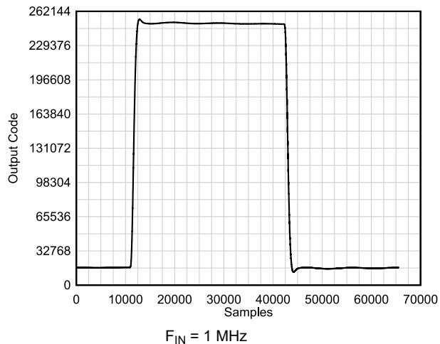
图 6-24. Pulse Response
