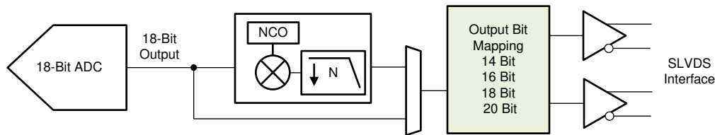
图 8-38. Interface output bit mapper
