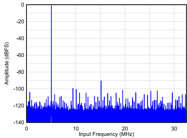
图 6-2. Single Tone FFT at F_{IN} = 5\text{ MHz}
