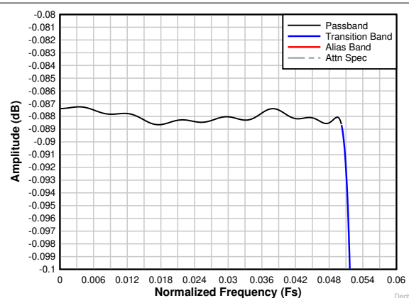
图 8-30. Decimation by 8 complex passband ripple response
