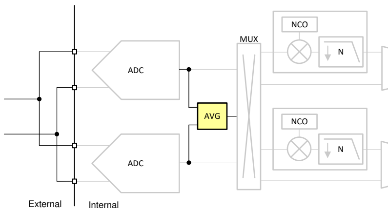
图 8-40. Digital Channel Averaging Diagram
