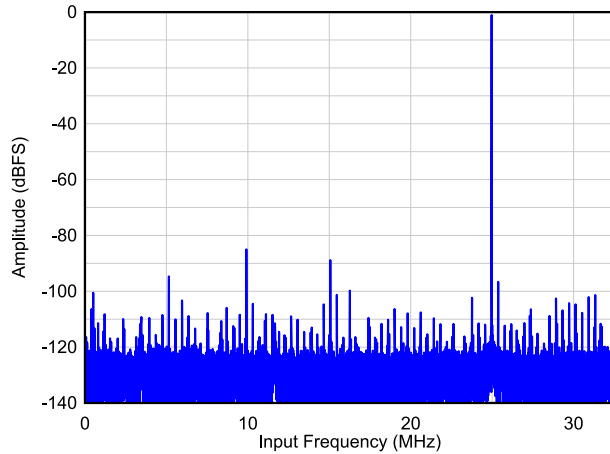
图 6-5. Single Tone FFT at F_{IN} = 40 MHz
