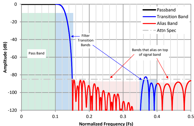
图 8-24. Interpretation of the Decimation Filter Plots
