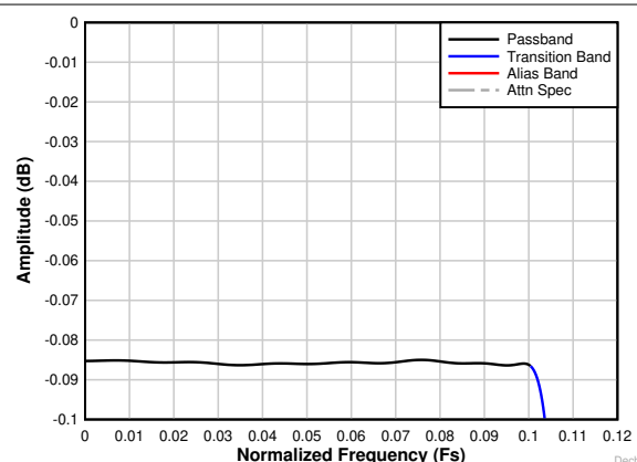
图 8-28. Decimation by 4 complex passband ripple response
