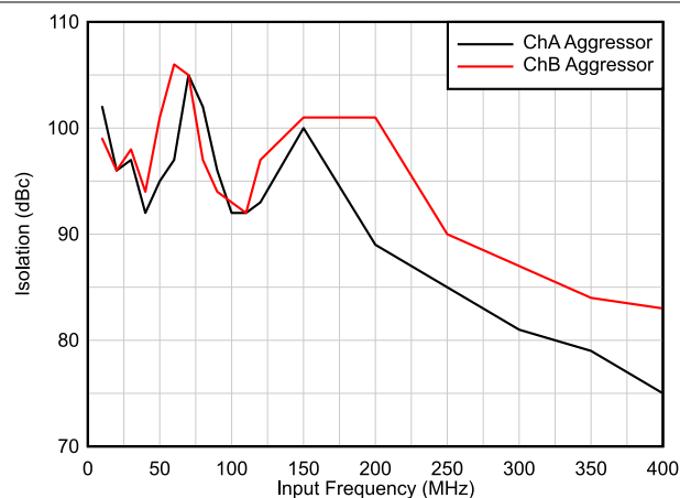
图 6-20. Isolation vs Input Frequency
