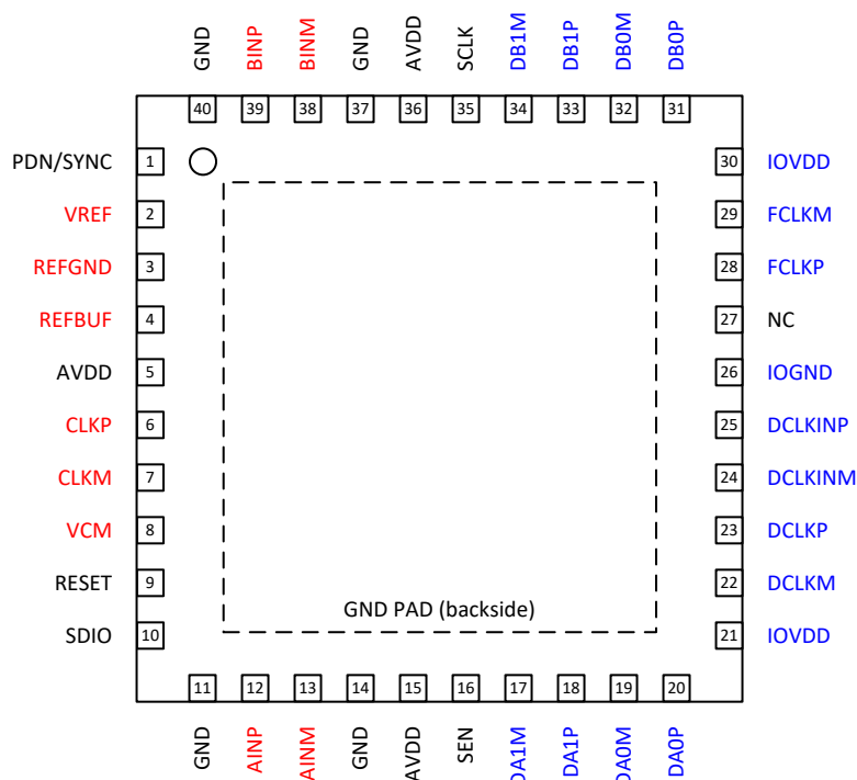
图 5-1. RSB Package, 40-Pin WQFN, Top View
