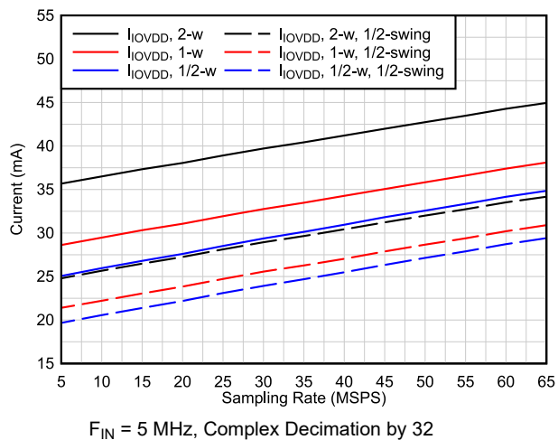
图 6-27. I_{OVDD} Current vs Output Interface
