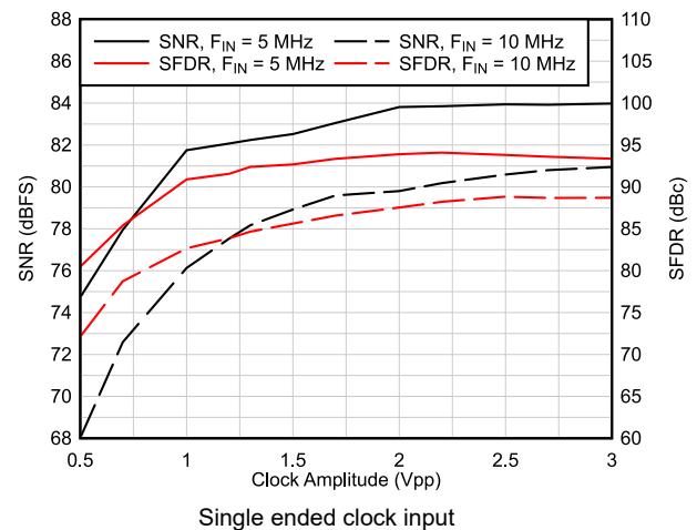
图 6-16. AC Performance vs Clock Amplitude
