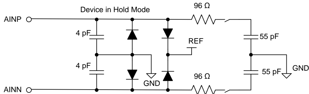
Figure 47. Input Sampling Stage Equivalent Circuit
