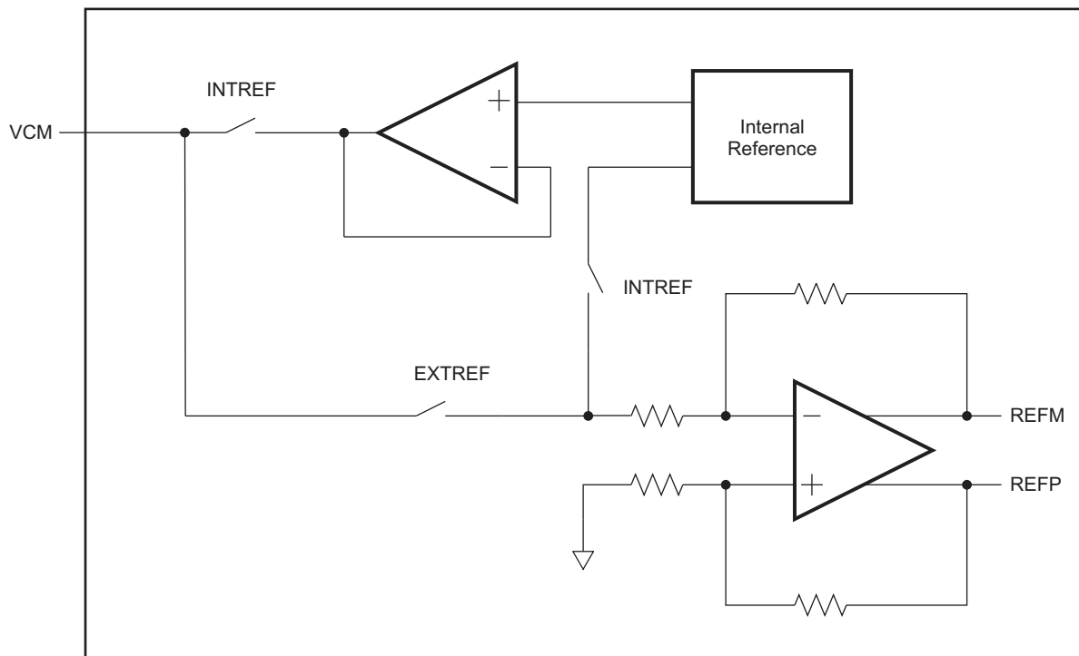
Figure 106. Reference Section
