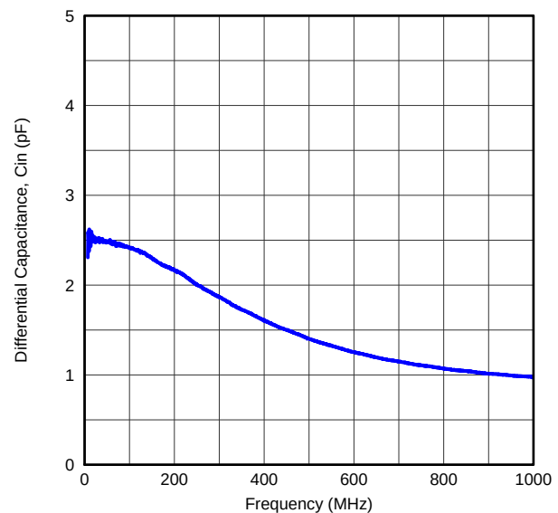
Figure 56. ADC Analog Input Capacitance ( C_{IN} ) Across Frequency
