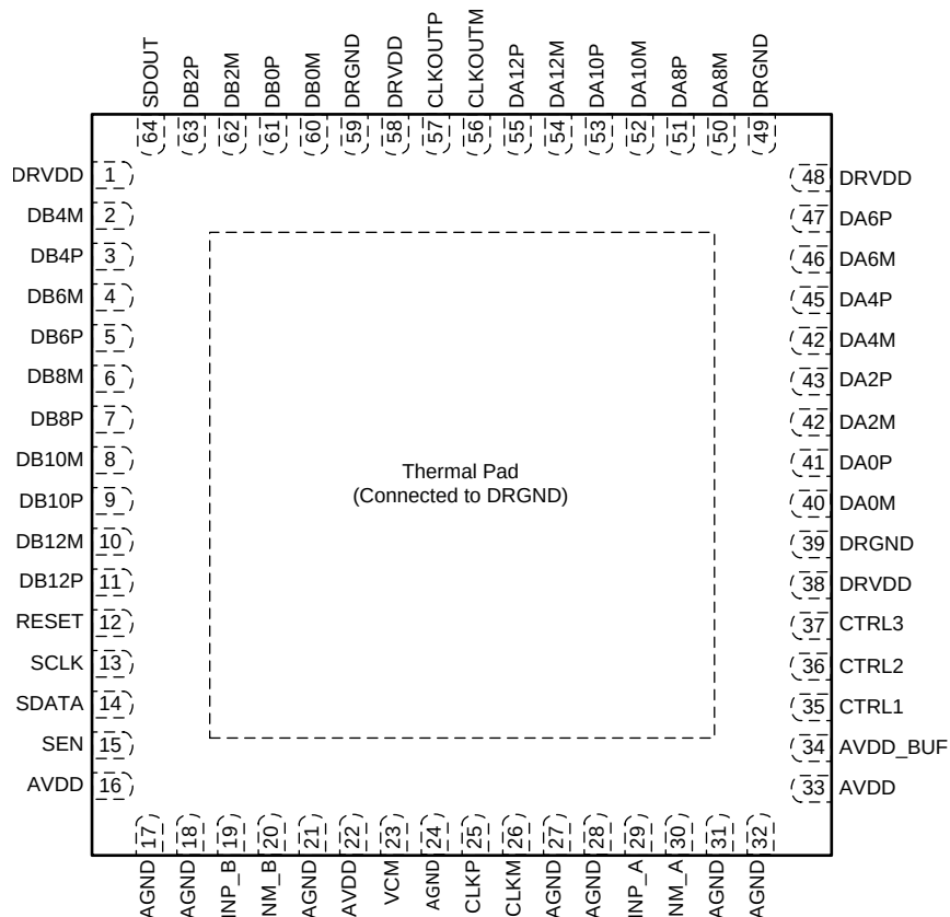
RGC Package (1) 64-Pin VQFN With Exposed Thermal Pad LVDS Mode - Top View
