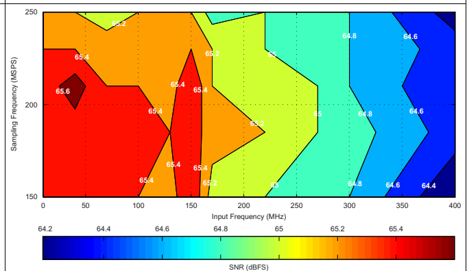
Figure 36. Signal-to-Noise Ratio (6-dB Gain)
