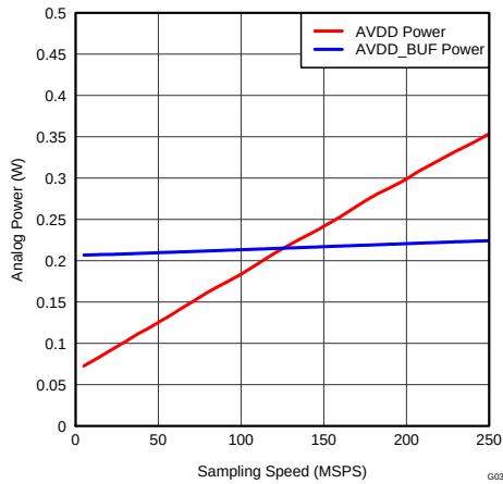
Figure 31. Analog Power vs Sampling Frequency
