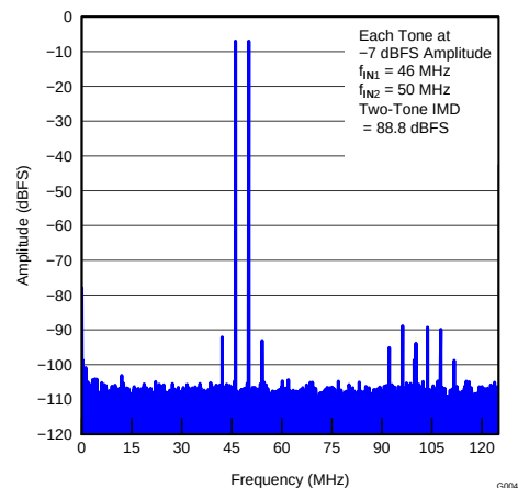
Figure 4. Two-Tone Input Signal
