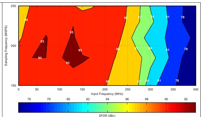
Figure 34. Spurious-Free Dynamic Range (6-dB Gain)
