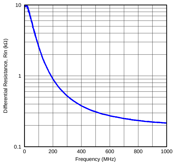
Figure 55. ADC Analog Input Resistance ( R_{IN} ) Across Frequency
