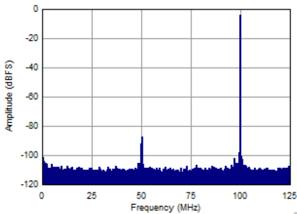
Figure 63. 100-MHz Input Frequency
