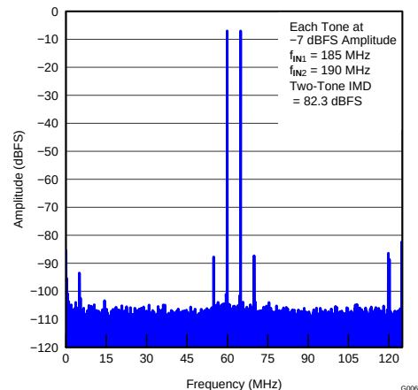
Figure 6. Two-Tone Input Signal
