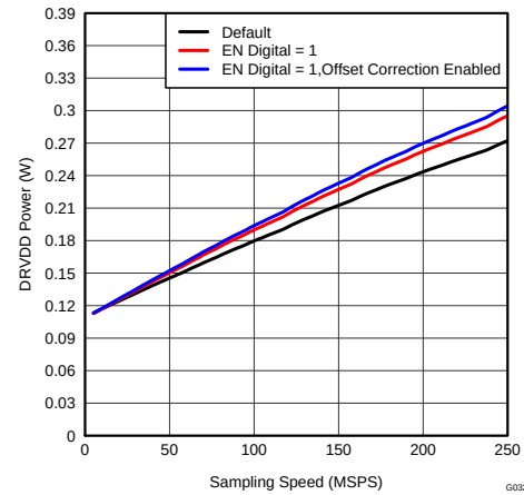
Figure 32. Digital Power vs Sampling Frequency
