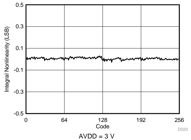
Figure 17. Typical INL
