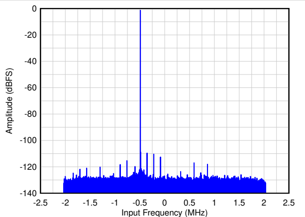
图 9-3. Single Tone FFT at F_{IN} = 5 MHz
