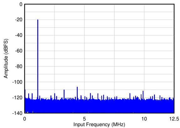
图 6-23. Single Tone FFT at F_{IN} = 1.1 \text{ MHz}
