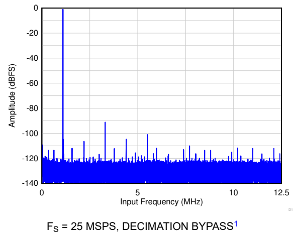
图 6-22. Single Tone FFT at F_{IN} = 1.1 \text{ MHz}
