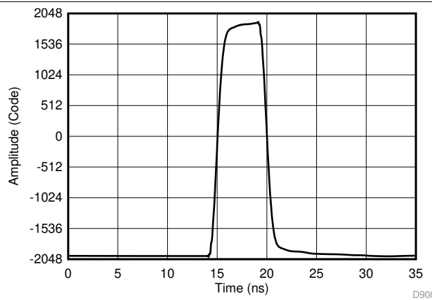
图 93. Measured Pulse using Sub-Sampling Technique for Equivalent 32 GSPS Measurement
