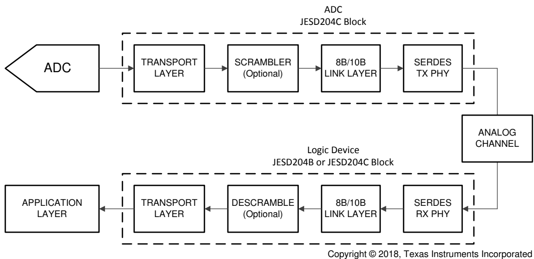
图 7. Simplified 8B/10B Encoded JESD204C Interface Diagram
