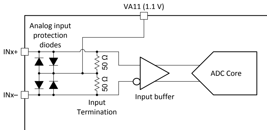
图 4. ADC12QJ1600-Q1 Analog Input Internal Termination and Protection Diagram
