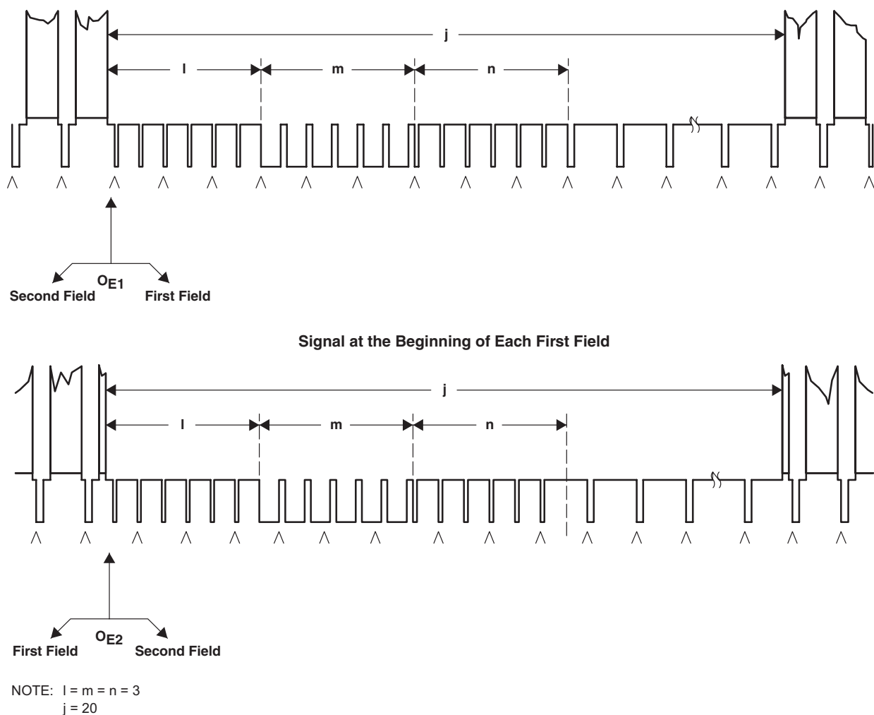
Figure 6-38. Field/Frame Synchronizing Signal Waveform (525I Format)
