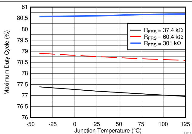
Figure 7-12. Maximum Duty Cycle vs Temperature
