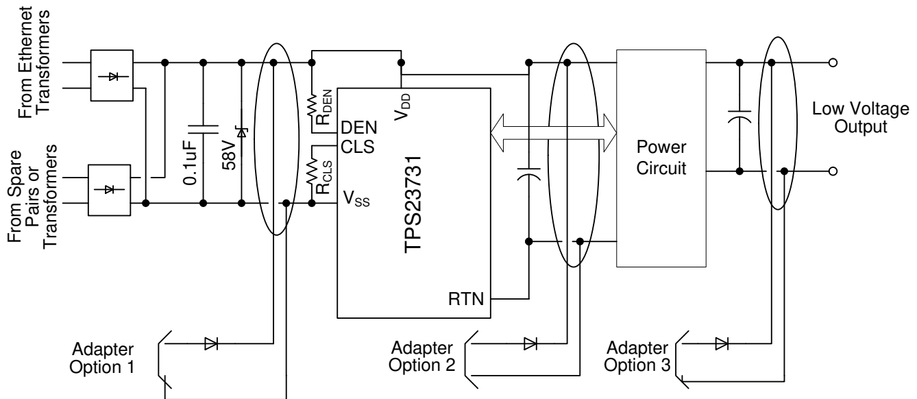
Figure 8-15. ORing Configurations
