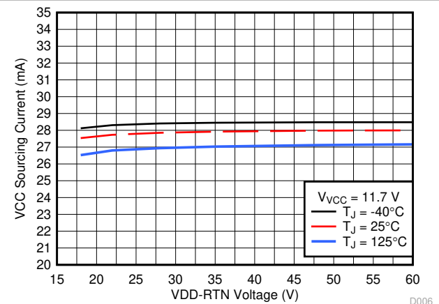
Figure 7-5. Converter Startup Current vs VDD Input Voltage
