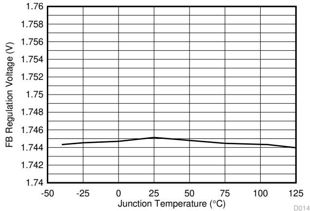
Figure 7-13. Feedback Regulation Voltage vs Temperature
