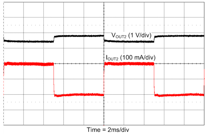
Figure 32. Load Transient at I_{OUT2} = 100\text{ mA} - 300\text{mA}
