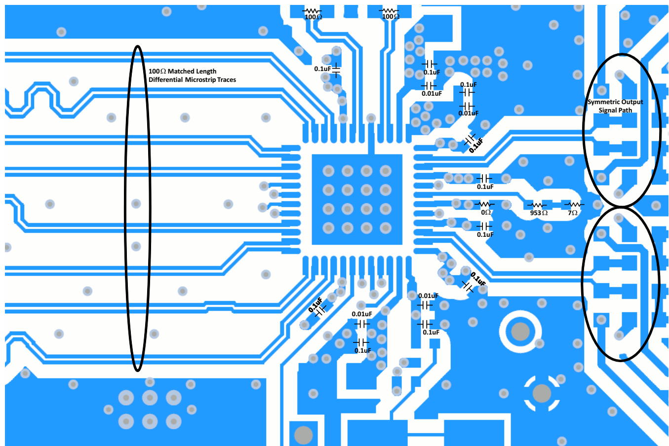
Figure 93. Layout Example
