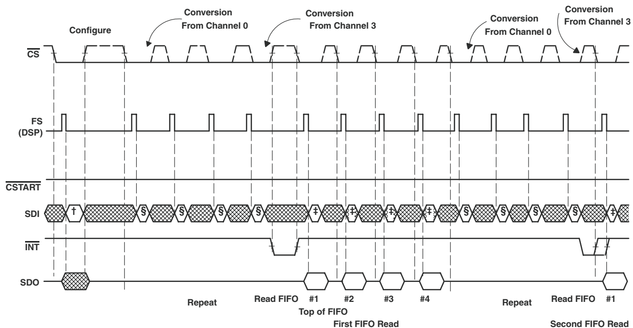
Figure 11. TLV2548 Mode 01 µp/DSP Serial Interface (Conversions Triggered by CSTART)
