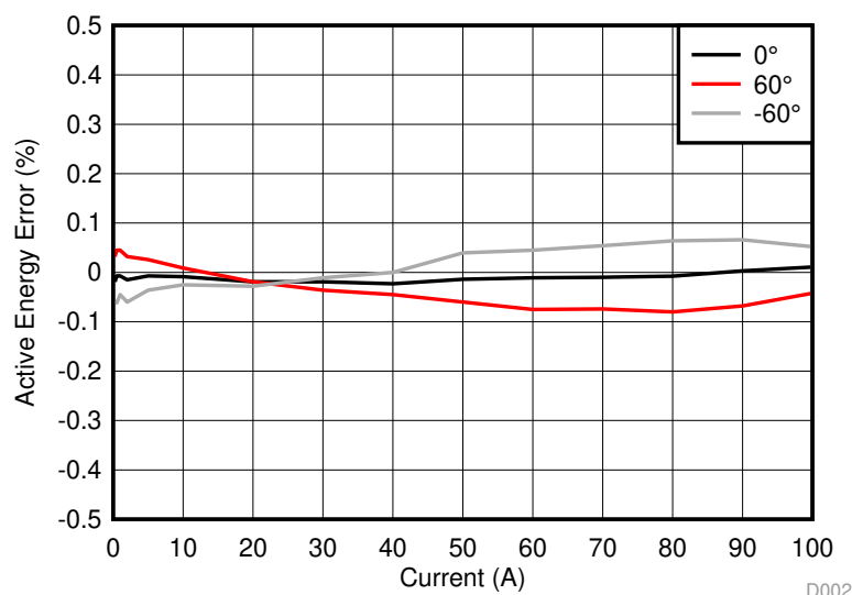
图 90. Phase B Active Energy % Error Versus Current
