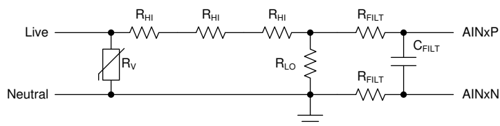
图 87. Voltage Measurement Front-End
