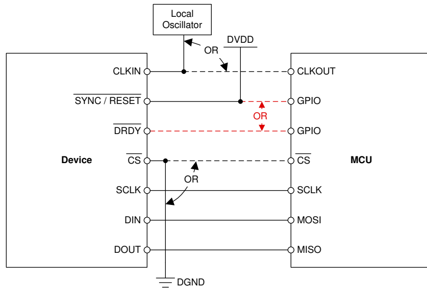
图 80. Minimum Connections Required to Operate the ADS131M04
