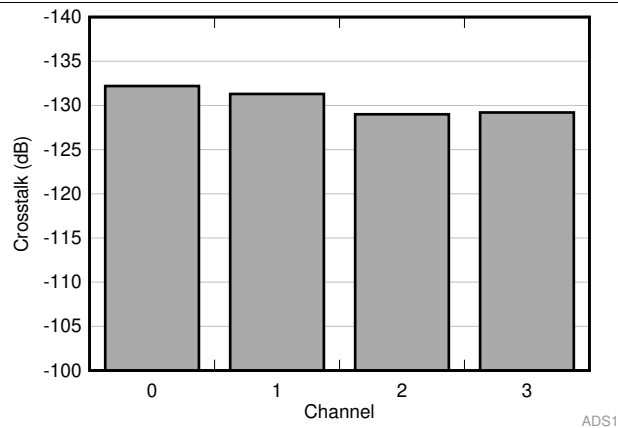
图 16. Crosstalk vs Channel
