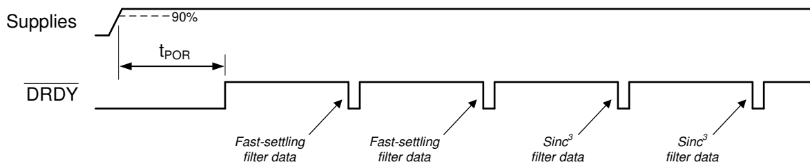
图 37. Fast-Settling Behavior
