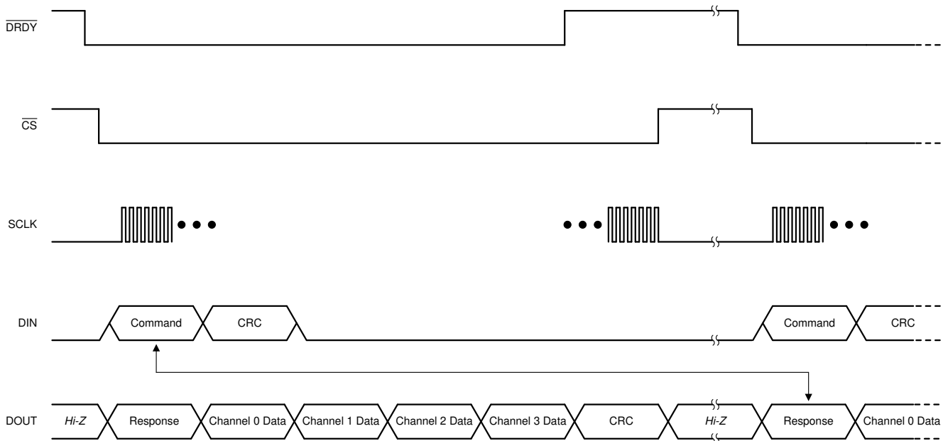
图 40. Typical Communication Frame
