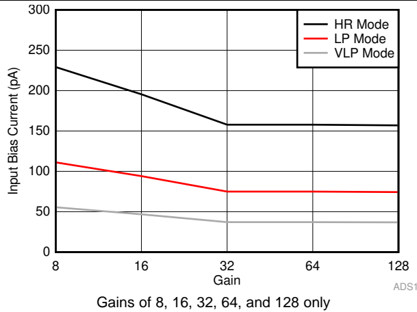
图 4. Input Bias Current vs Gain
