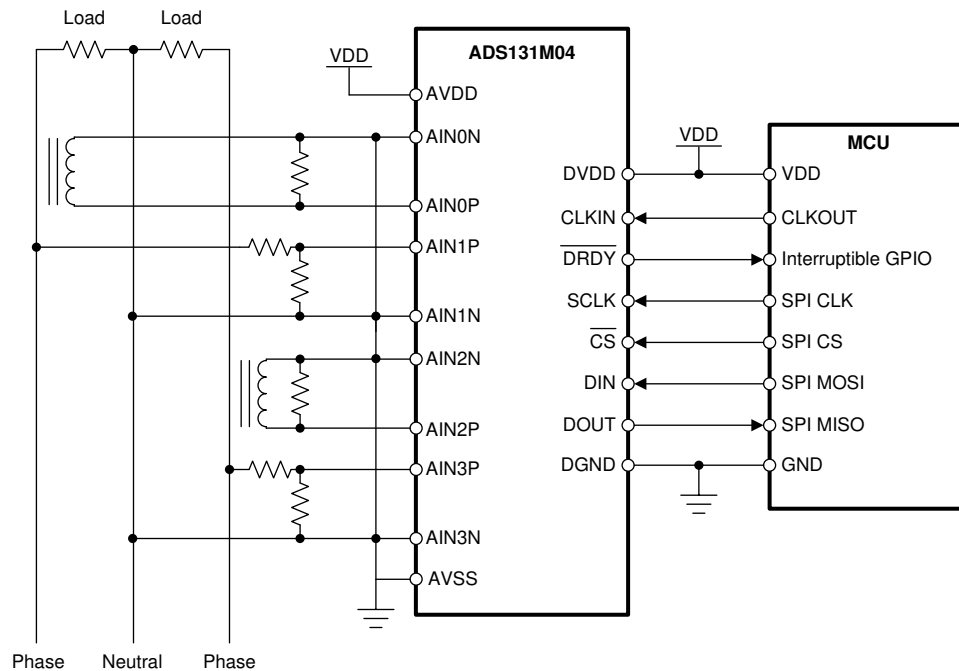
图 86. Split-Phase Metrology Design Front-End
