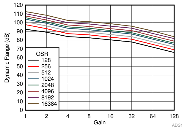
图 13. Dynamic Range at 4 kSPS vs Gain
