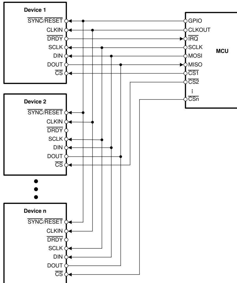
图 85. Multiple Device Configuration
