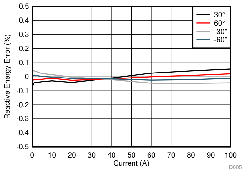
图 92. Cumulative Reactive Energy % Error Versus Current
