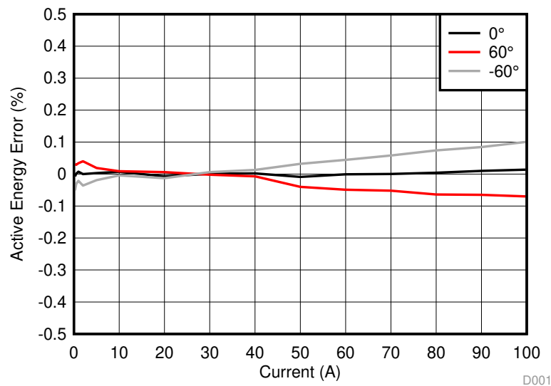
图 89. Phase A Active Energy % Error Versus Current
