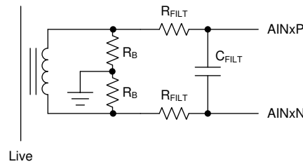
图 88. Current Measurement Front-End
