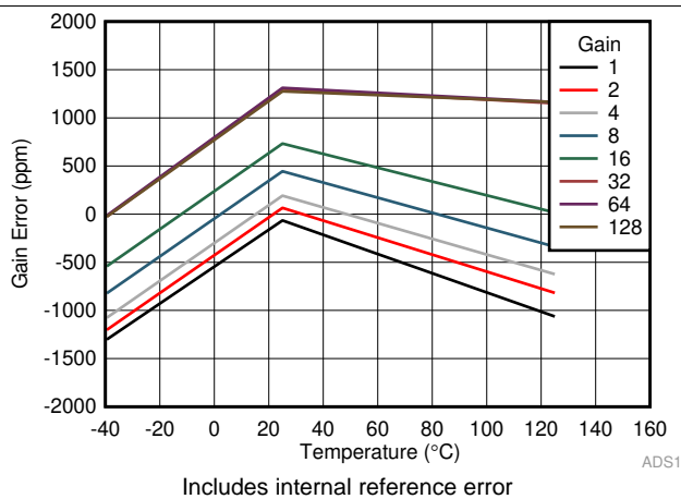
图 8. Gain Error vs Temperature
