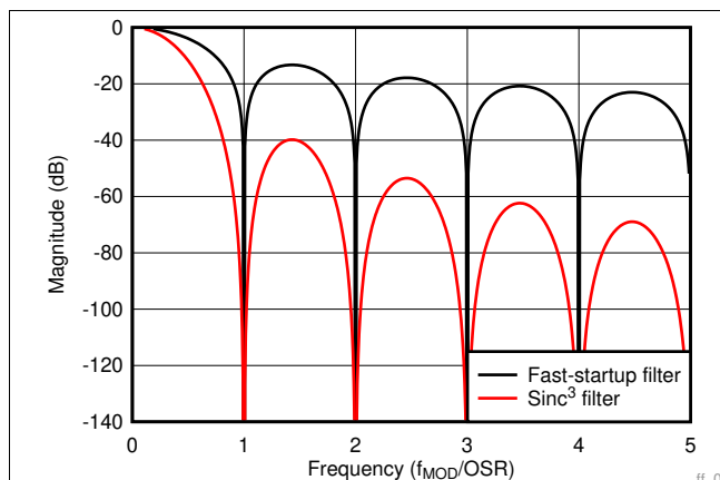
图 29. Fast-Settling and Sinc 3 Digital Filter Response
