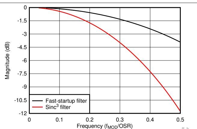
图 30. Fast-Settling and Sinc 3 Digital Filter Response, Pass-Band Detail
