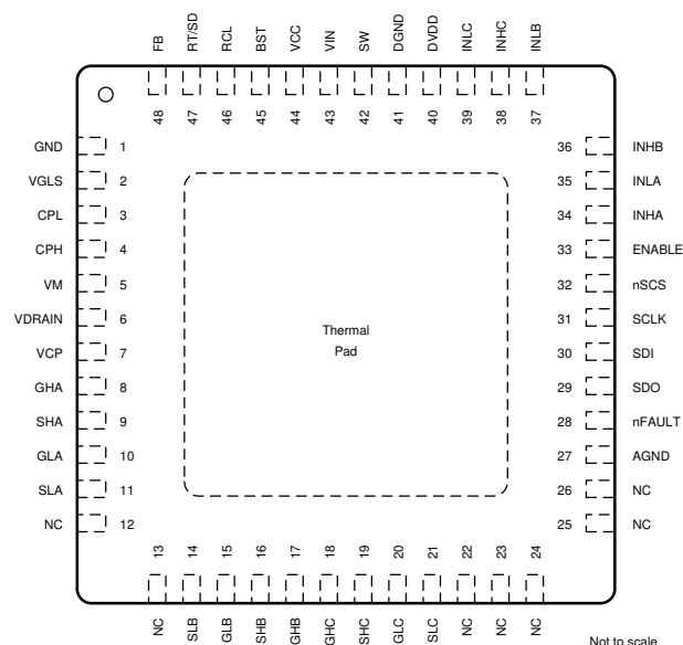
Figure 6-4. DRV8350RFS RGZ Package 48-Pin VQFN With Exposed Thermal Pad Top View
