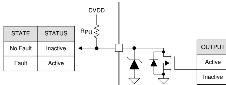
Figure 8-27. Open-Drain Output Pin Structure
