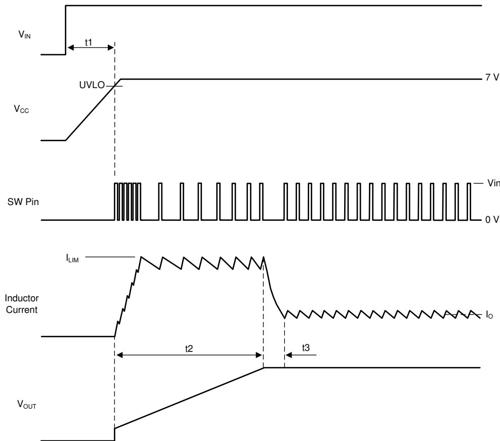
Figure 8-39. Start-Up Sequence
