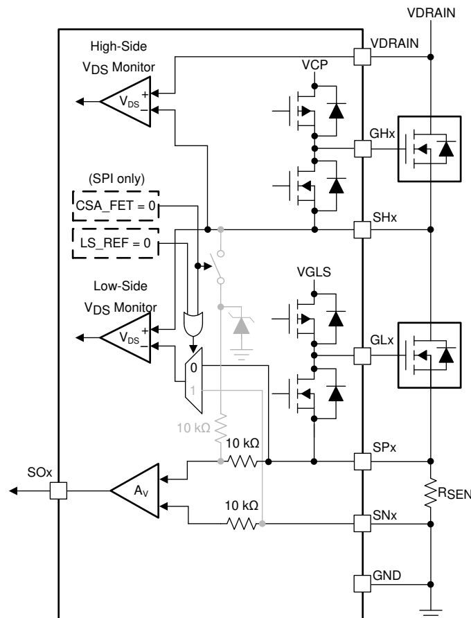
Figure 8-35. Resistor Sense Configuration
