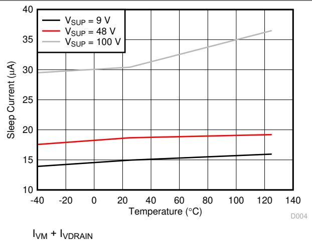
Figure 7-4. Sleep Current Over Temperature
