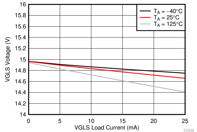
Figure 7-8. VGLS Voltage Over Load Current
