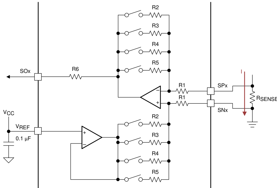
Figure 8-31. Unidirectional Current-Sense Configuration
