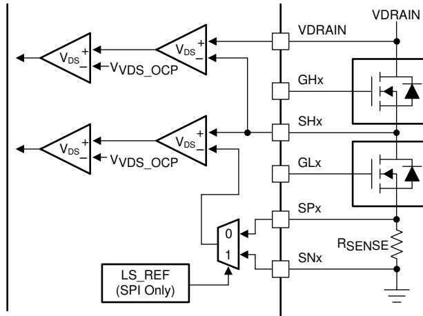
Figure 8-22. DRV8353F and DRV8353RF V_{DS} Monitors
