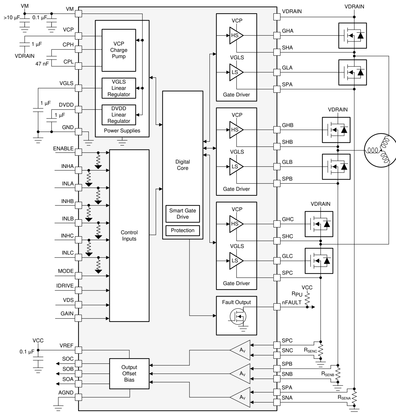
Figure 8-5. Block Diagram for DRV8353FH
