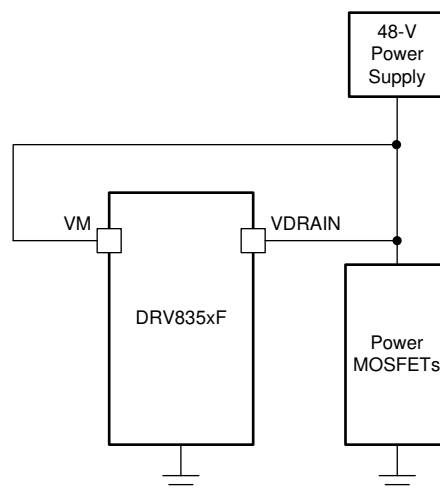
Figure 8-17. Single Supply Example
