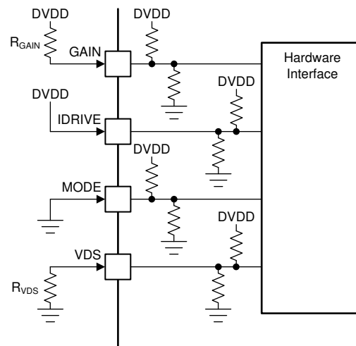
Figure 8-15. Hardware Interface
