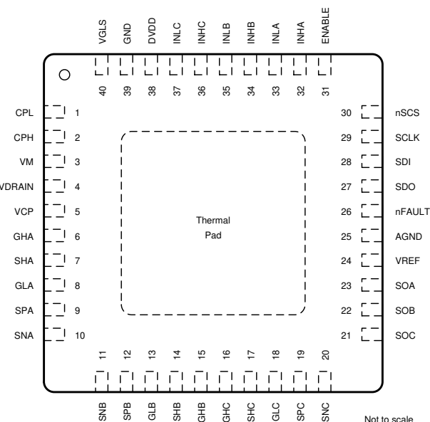
Figure 6-6. DRV8353FS RTA Package 40-Pin WQFN With Exposed Thermal Pad Top View
