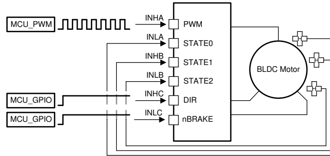
Figure 8-10. 1x PWM—Hall Sensor
