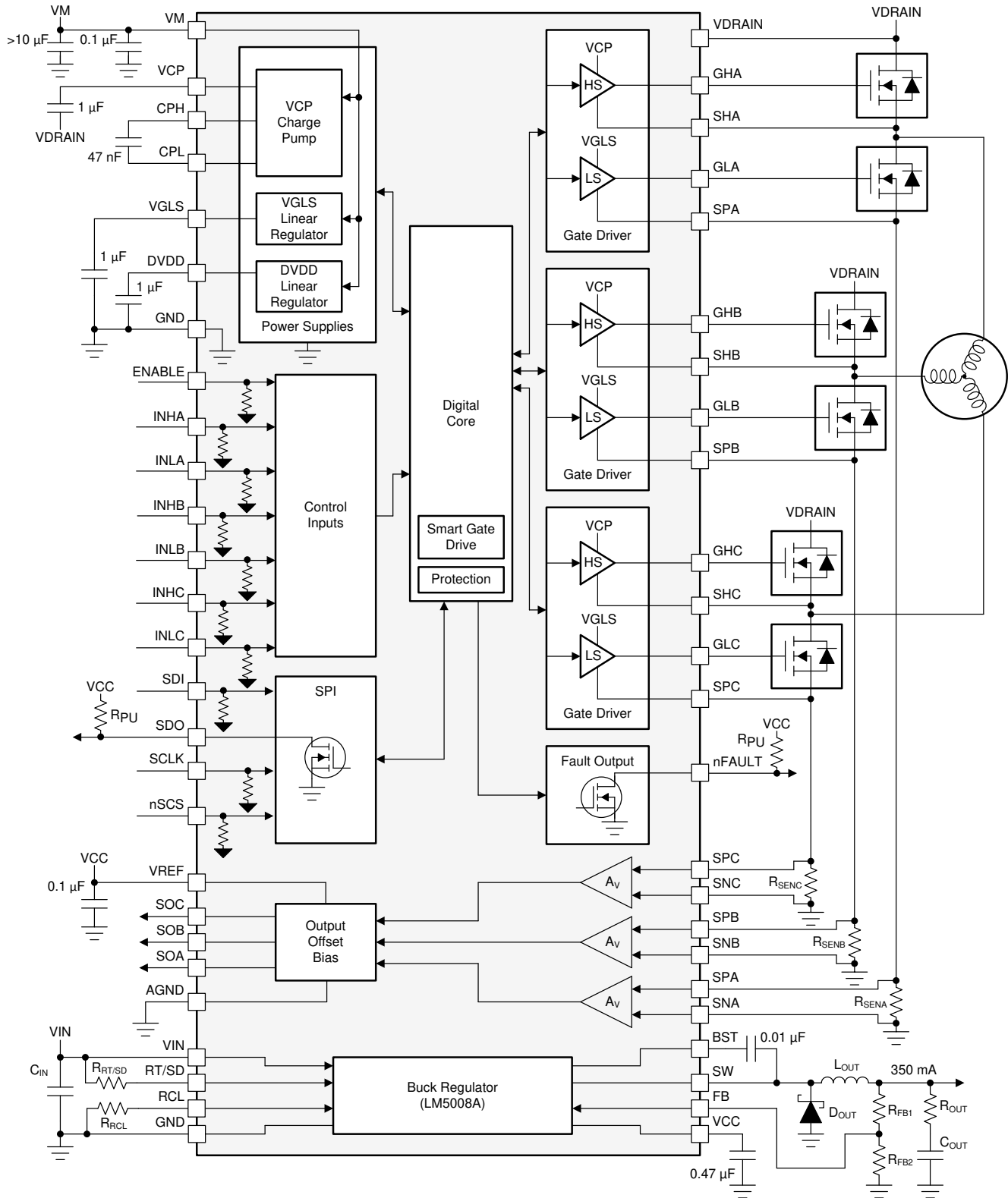
Figure 8-8. Block Diagram for DRV8353RFS
