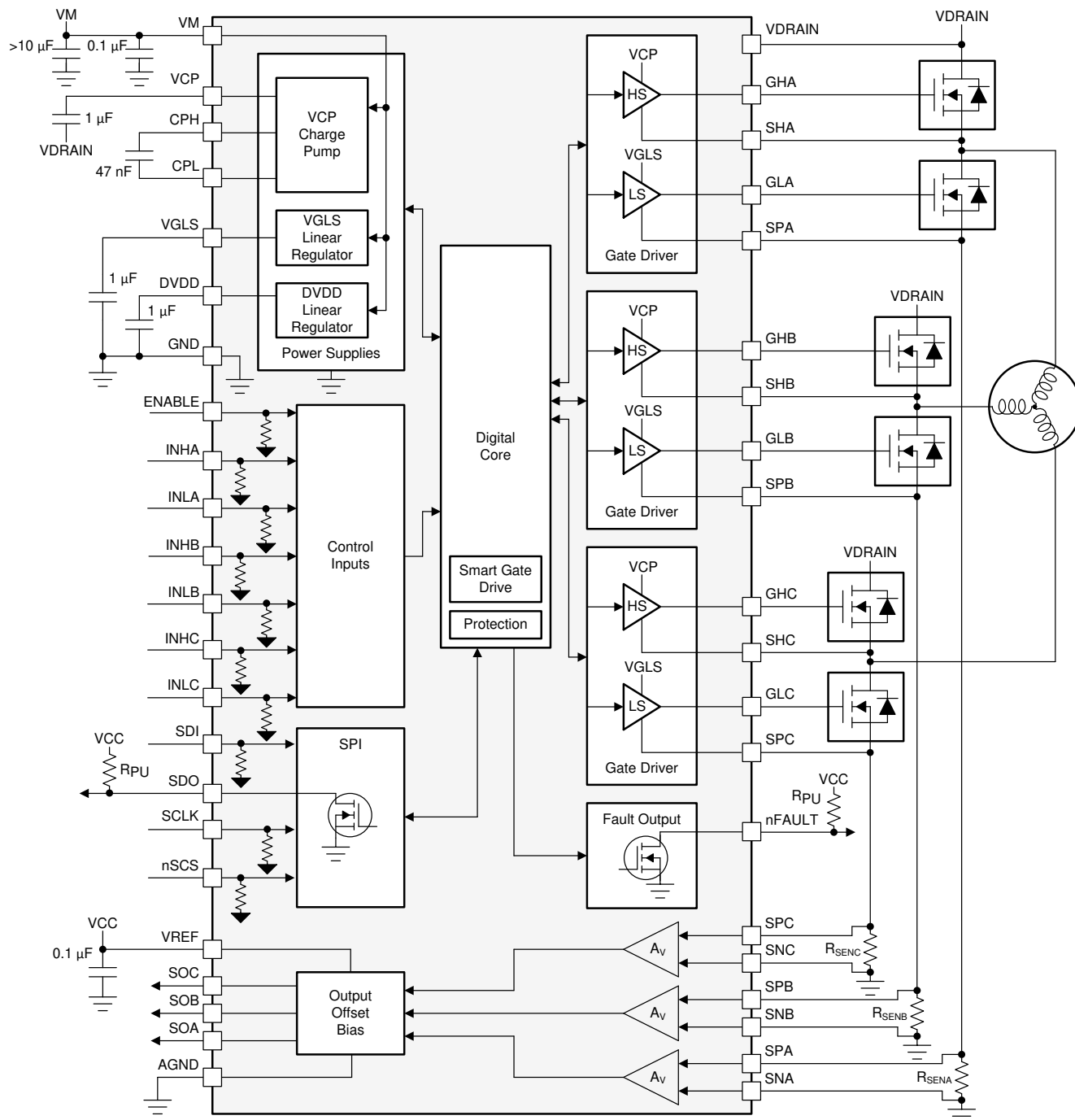
Figure 8-6. Block Diagram for DRV8353FS
