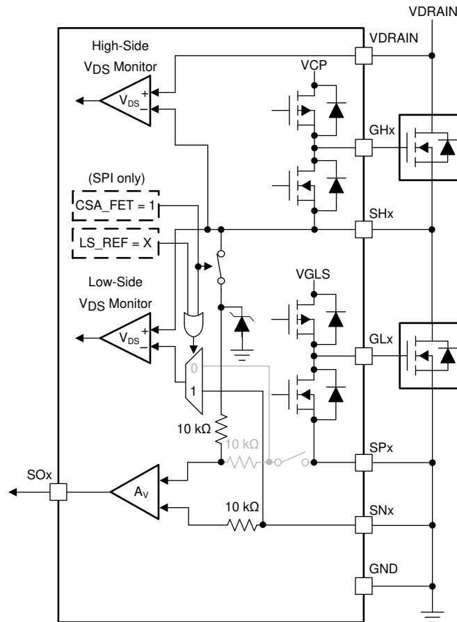
Figure 8-36. V_{DS} Sense Configuration
