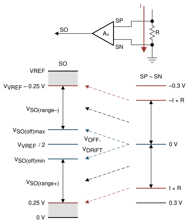
Figure 8-30. Bidirectional Current Sense Regions
