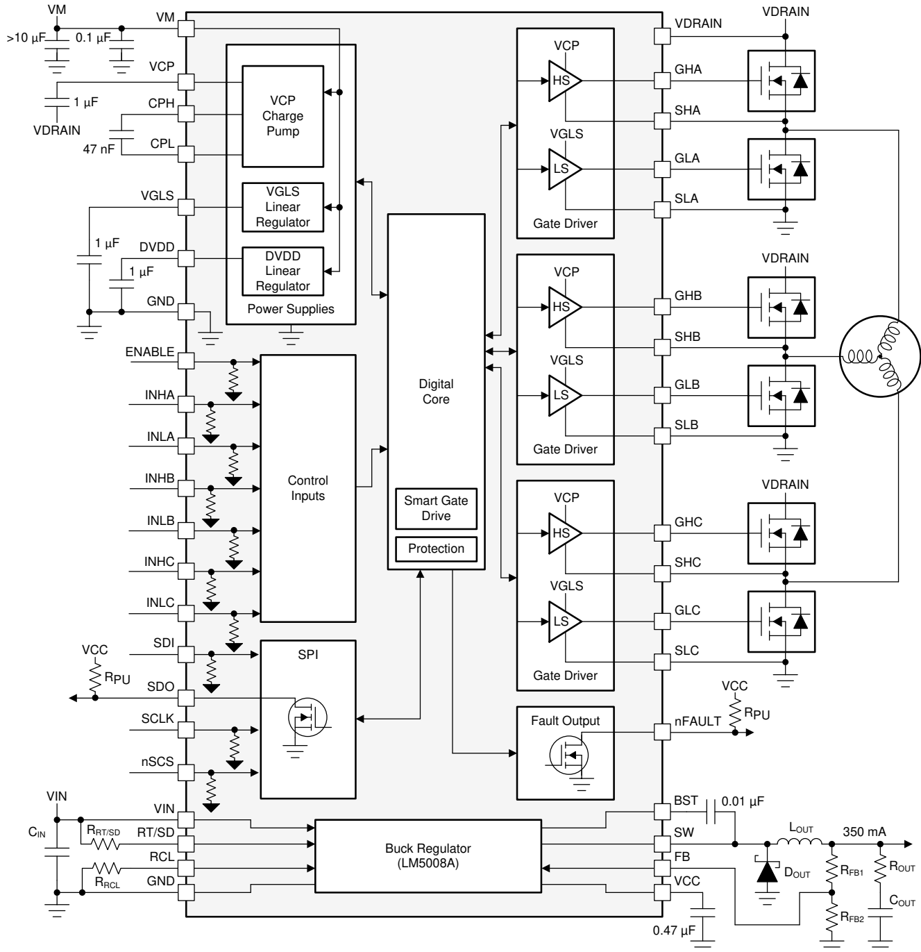
Figure 8-4. Block Diagram for DRV8350RFS
