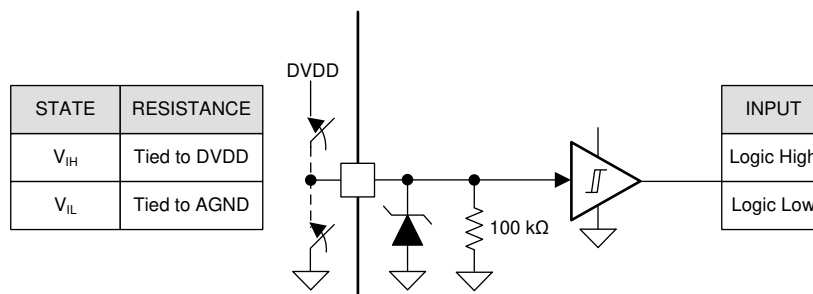
Figure 8-24. Logic-Level Input Pin Structure
