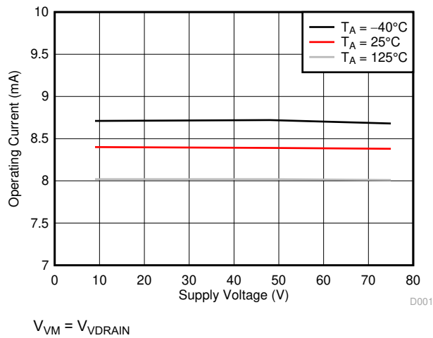
Figure 7-1. VM Supply Current Over Supply Voltage
