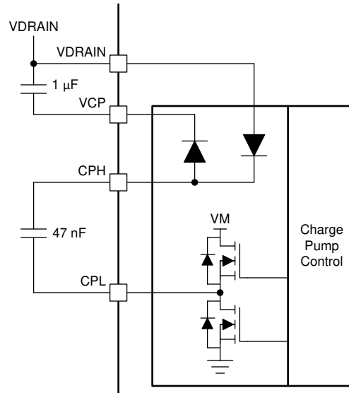
Figure 8-16. Charge Pump Architecture
