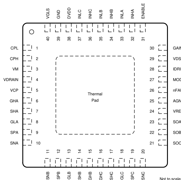
Figure 6-5. DRV8353FH RTA Package 40-Pin WQFN With Exposed Thermal Pad Top View
