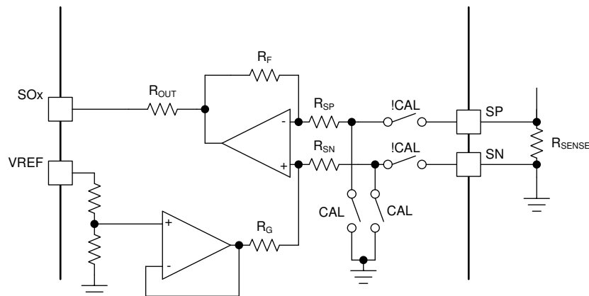
Figure 8-34. Amplifier Manual Calibration
