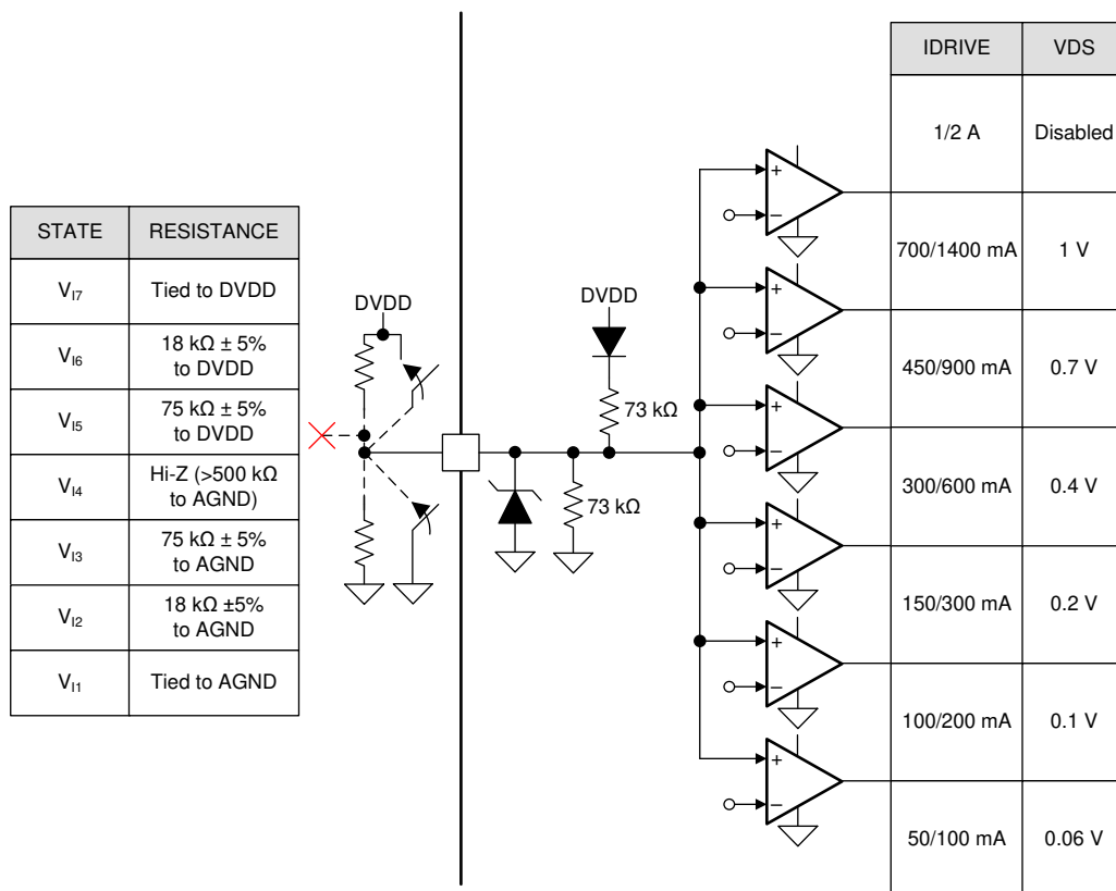
Figure 8-26 shows the structure of the seven level input pins, IDRIVE and VDS, on hardware interface devices. The input can be set with an external resistor.
