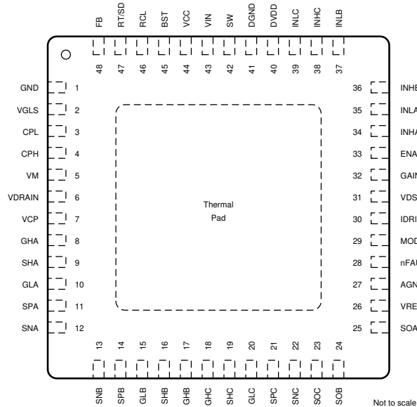
Figure 6-7. DRV8353RFH RGZ Package 48-Pin VQFN With Exposed Thermal Pad Top View
