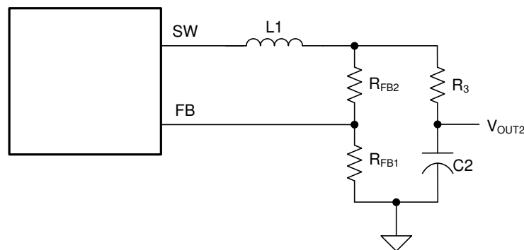
Figure 8-38. Low-Ripple Output Configuration
