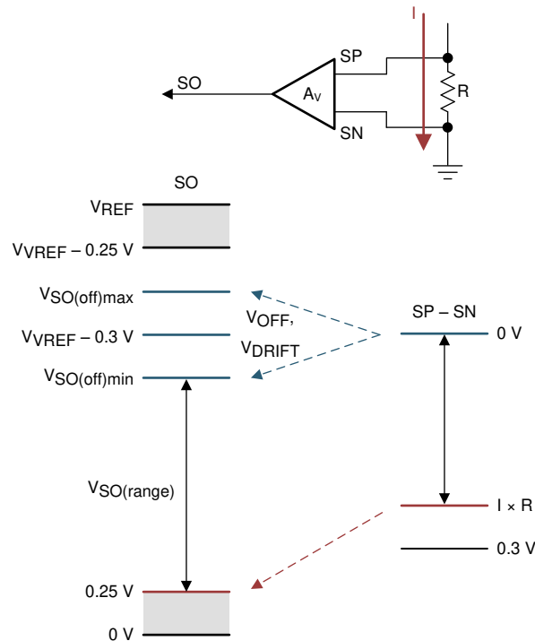
Figure 8-33. Unidirectional Current-Sense Regions
