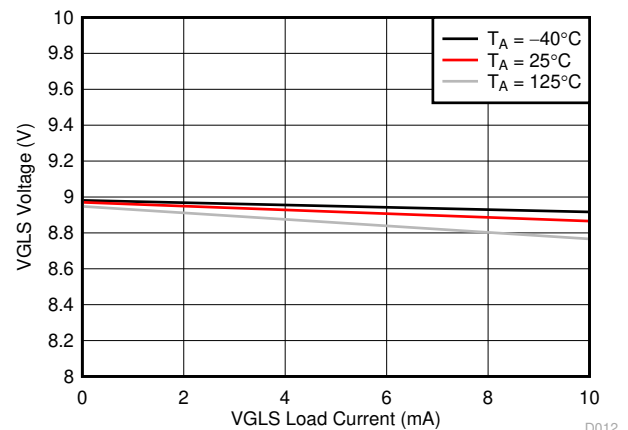
Figure 7-10. VGLS Voltage Over Load Current
