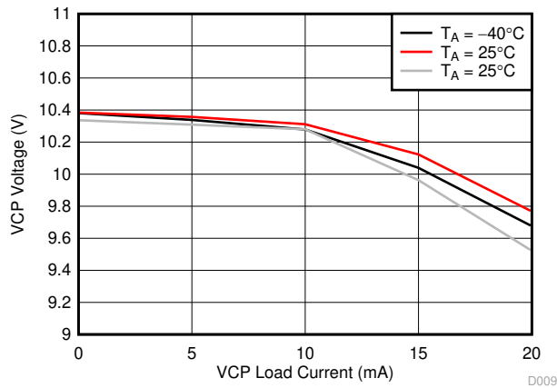
Figure 7-7. VCP Voltage Over Load Current
