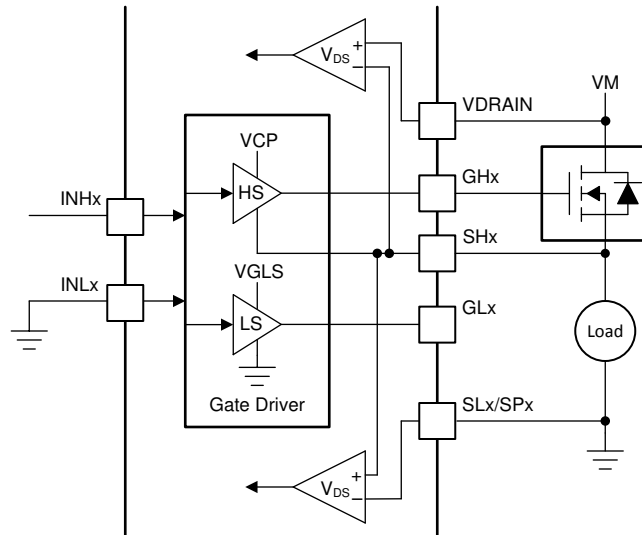
Figure 8-12. Single High-Side Driver
