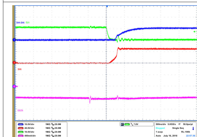
Figure 9-6. IDRIVE 300-mA and 600-mA Setting Positive Current
