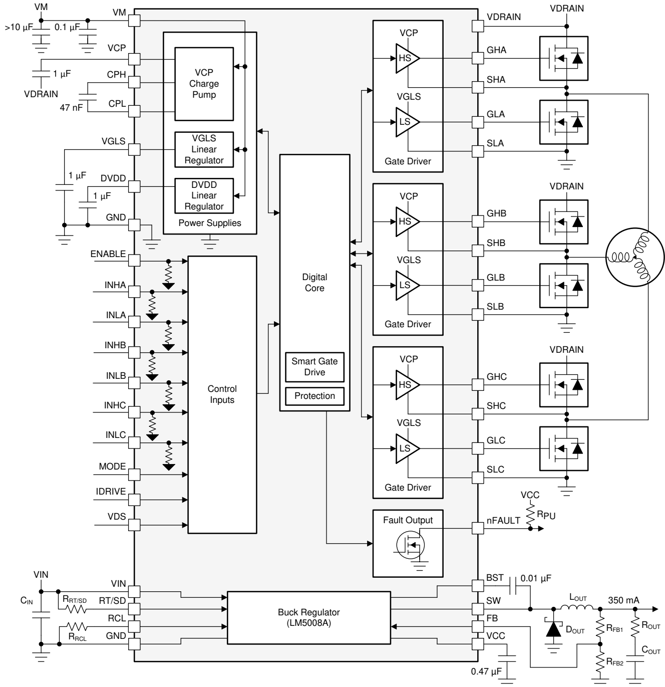
Figure 8-3. Block Diagram for DRV8350RFH
