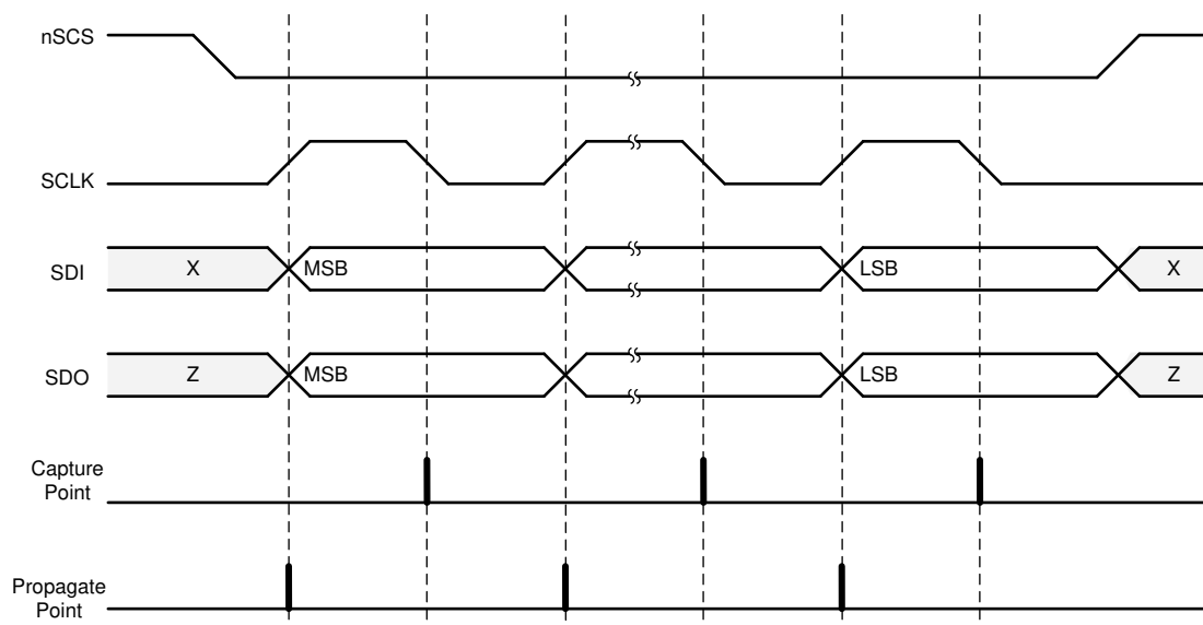
Figure 8-41. SPI Slave Timing Diagram
