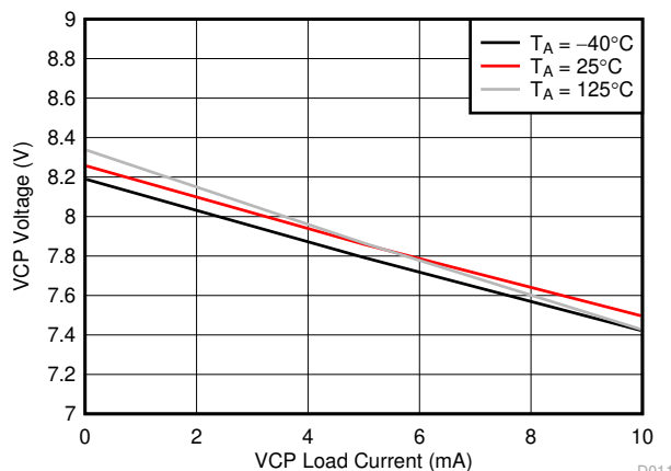
Figure 7-9. VCP Voltage Over Load Current
