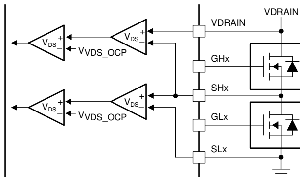
Figure 8-21. DRV8350F and DRV8350RF V_{DS} Monitors
