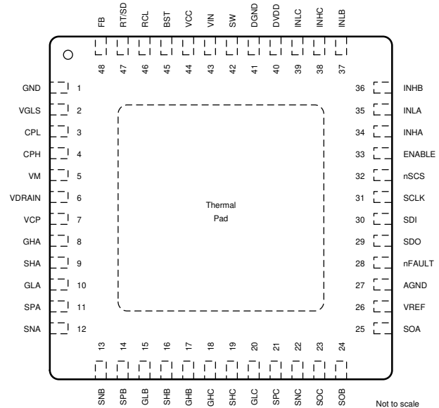
Figure 6-8. DRV8353RFS RGZ Package 48-Pin VQFN With Exposed Thermal Pad Top View
