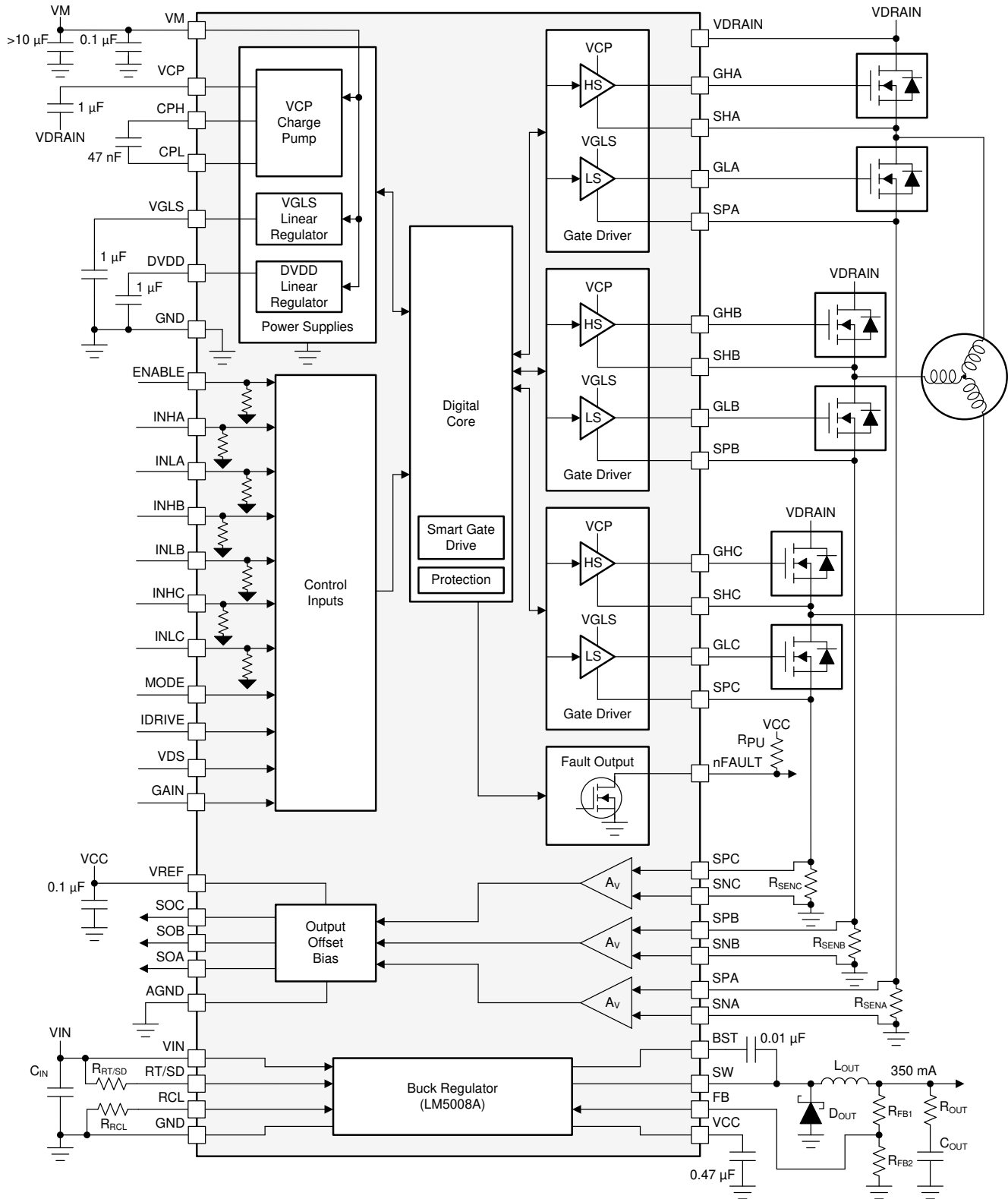
Figure 8-7. Block Diagram for DRV8353RFH
