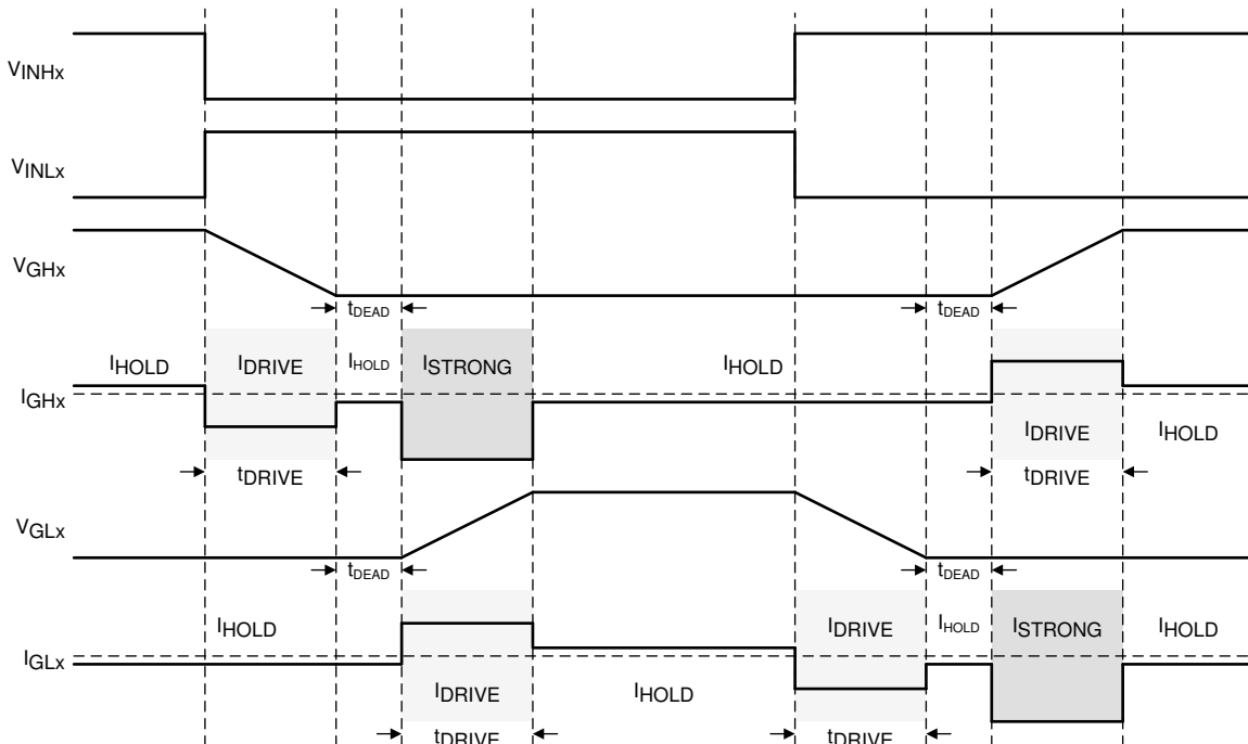
Figure 8-20. TDRIVE State Machine
