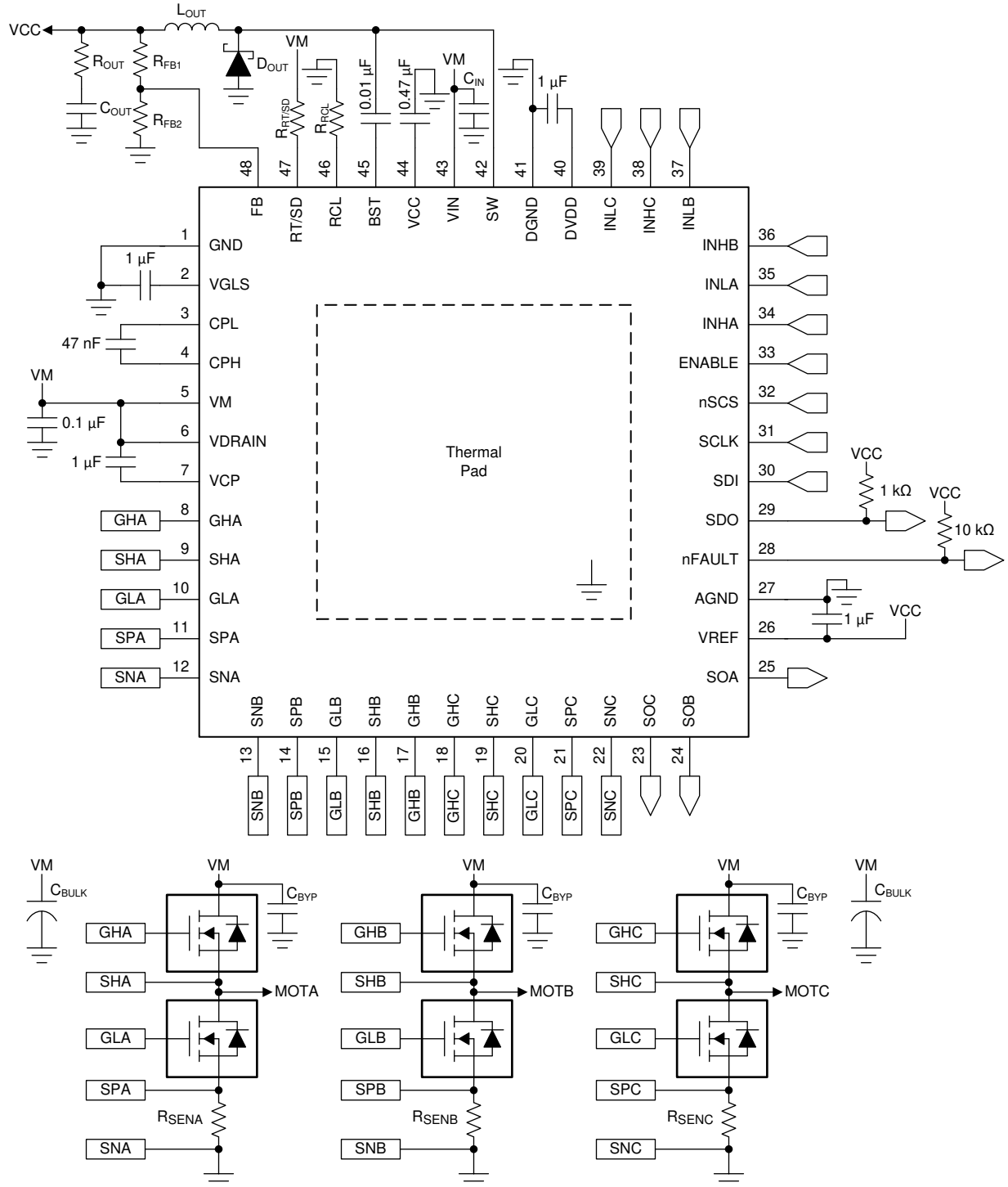
Figure 9-1. Primary Application Schematic
