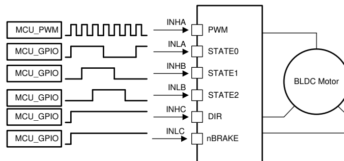
Figure 8-9. 1x PWM—Simple Controller
