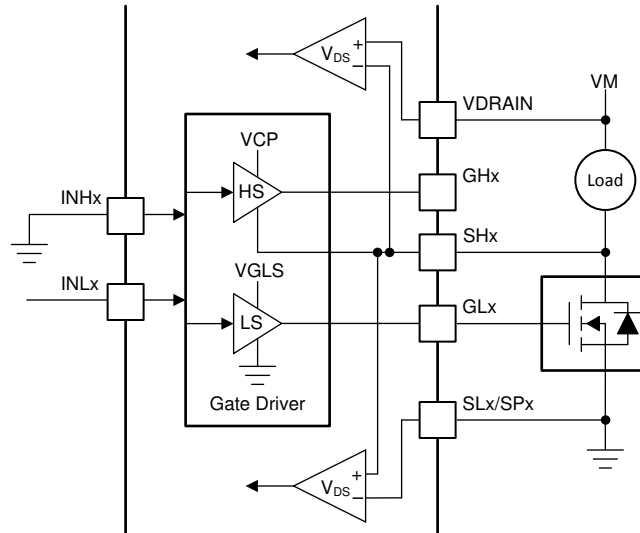
Figure 8-13. Single Low-Side Driver
