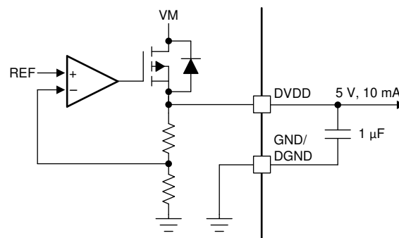
Figure 8-23. DVDD Linear Regulator Block Diagram
