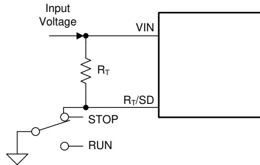
Figure 8-40. Shutdown Implementation
