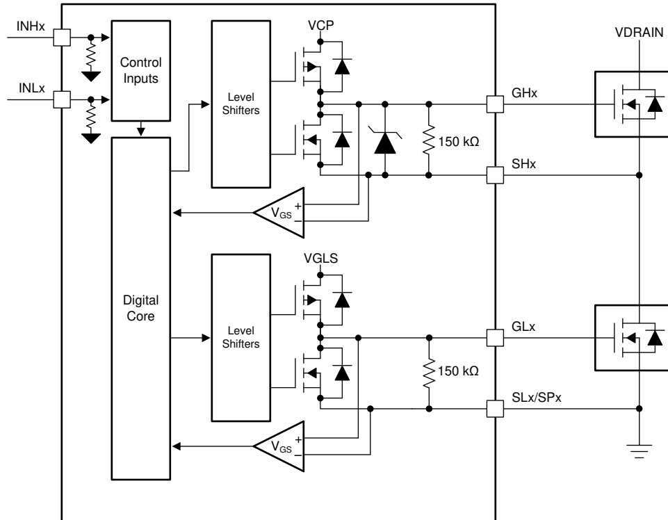
Figure 8-19. Gate Driver Block Diagram
