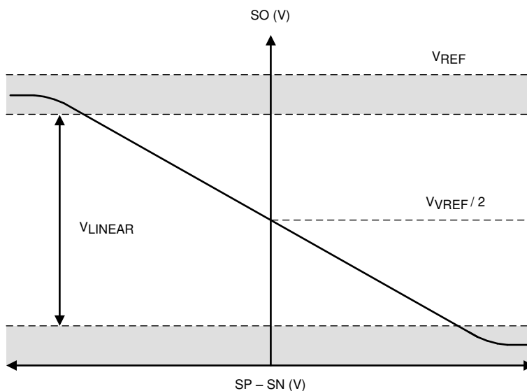
Figure 8-29. Bidirectional Current-Sense Output
