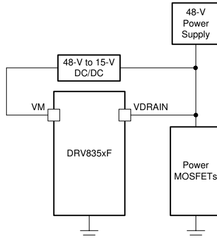
Figure 8-18. Dual Supply Example
