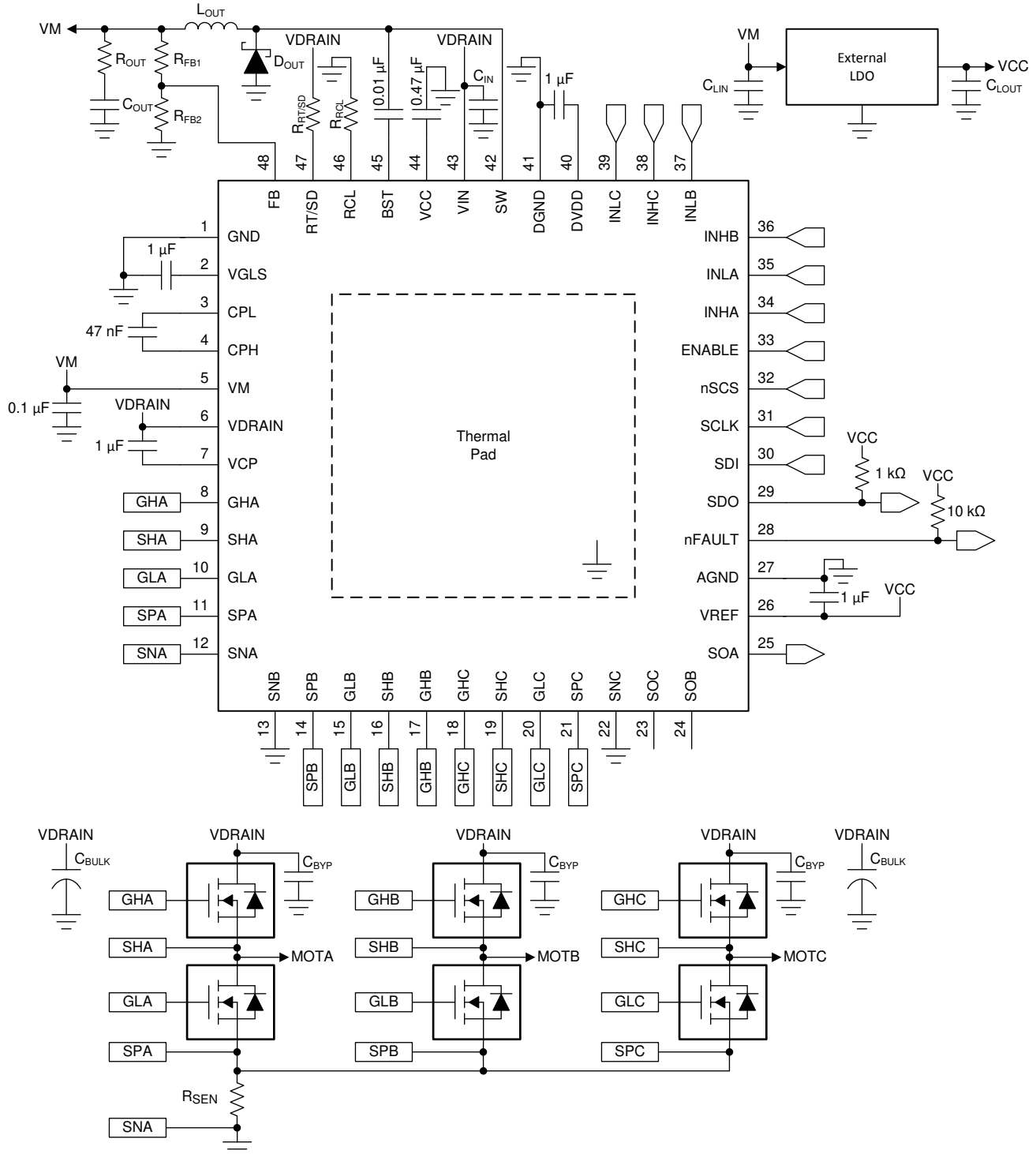
Figure 9-11. Alternative Application Schematic
