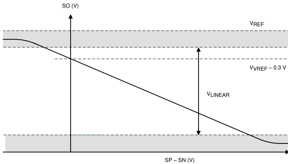
Figure 8-32. Unidirectional Current-Sense Output
