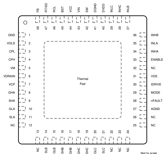
Figure 6-3. DRV8350RFH RGZ Package 48-Pin VQFN With Exposed Thermal Pad Top View
