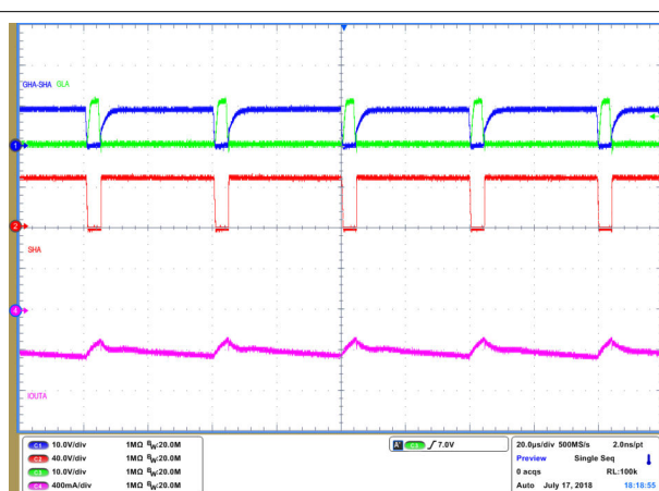
Figure 9-3. Gate Driver Operation 90% Duty Cycle
