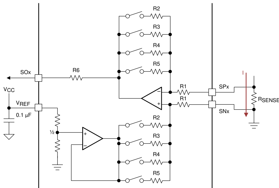
Figure 8-28. Bidirectional Current-Sense Configuration
