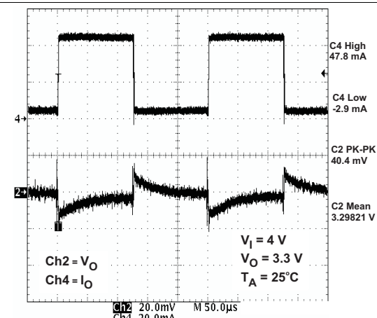
Figure 25. LDO2 Load Transient Response
