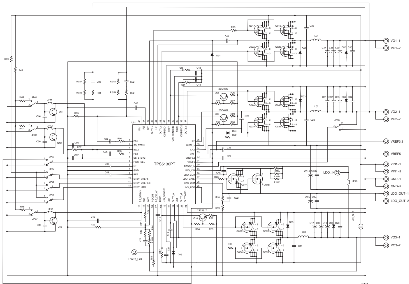
Figure 17. EVM Schematic
