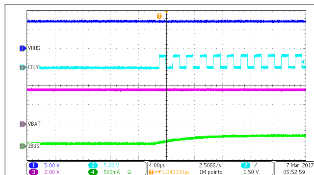
Figure 10-2. Power Up
