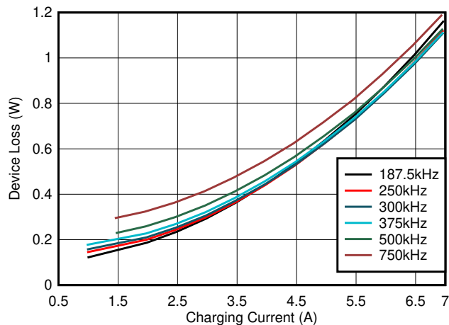
Figure 8-4. BQ25968 Device Power Loss, 4 x 22-μF Caps Per Phase
