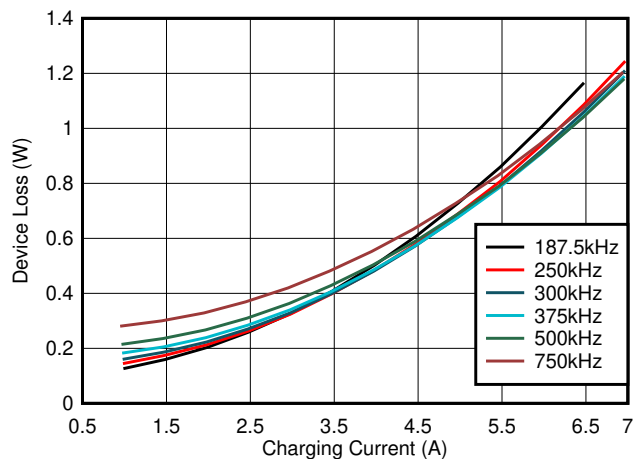
Figure 8-2. BQ25968 Device Power Loss, 4 x 20-μF Caps Per Phase
