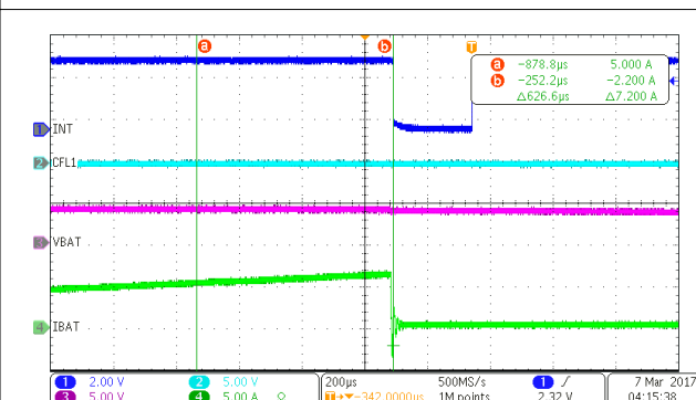
Figure 10-5. IBAT_OCP
