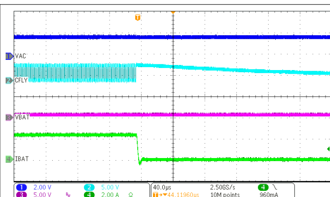
Figure 10-3. Disable Charge
