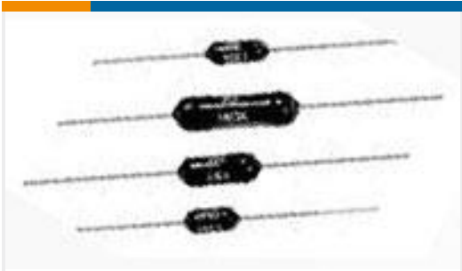
TE 产品编号2-1879639-8 H4P 36R5 0.5% 50PPM
