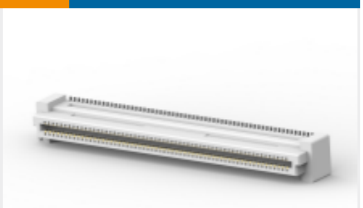
TE 产品编号1735482-5 Free Height Receptacle Conn: Board-Board, Vertical, 120, 0.8mm
