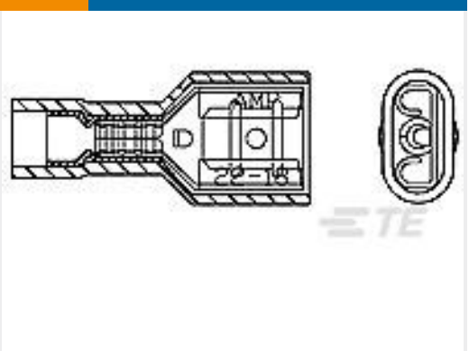
TE 产品编号735278 250 SERIES FASTON REC. PIDG
