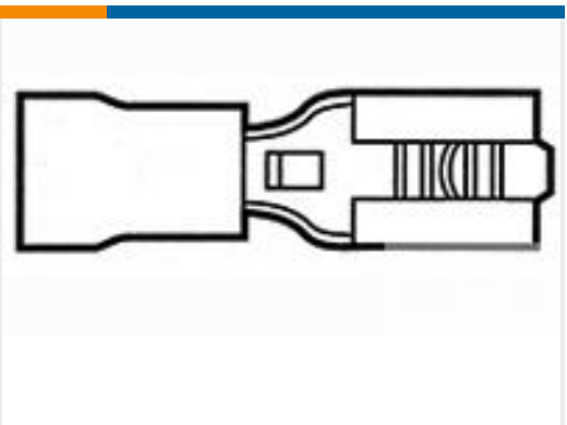
TE 产品编号184235-2 RECEPT, PIDG FASTON 16-14 187
