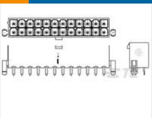
TE 产品编号2-1586040-0 20P VAL-U-LOK VRT HDR W/P V0
