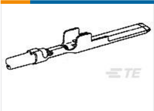
TE 产品编号170459-1 TAB WITH LANCE FOR M.I.C. L.P.
