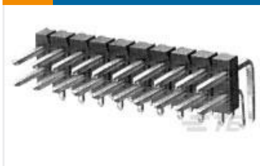
TE 产品编号1-825457-7 MOD 2 PINHDR 2X17P.
