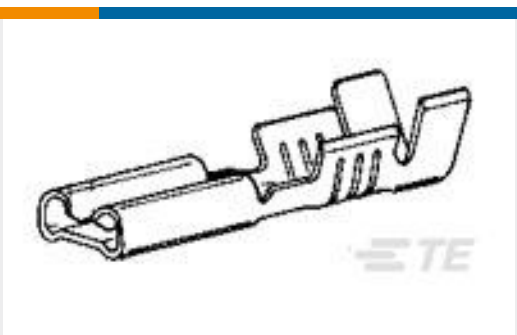
TE 产品编号140717-2 110 FASTON,REC.,22-18 AWG,PTBR
