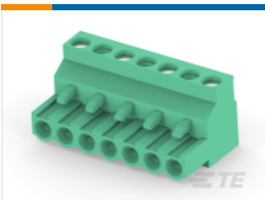
TE 产品编号1-282808-4 TERMI-BLOK PLUG STACKING 4P.10
