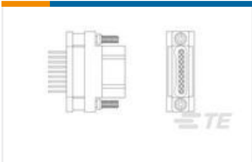
TE 产品编号1589461-8 SSM025C5N = THRU-HOLE
