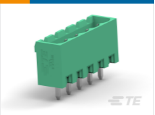
TE 产品编号1-2351885-4 14POS TB HDR 180 DEG, PITCH 5.0 &TL 4.5mm
