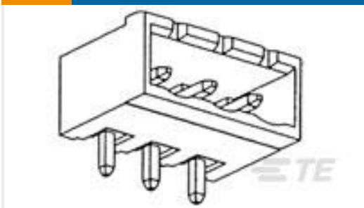
TE 产品编号1-796644-0 10POS 5.0MM CE R/A HDR,TRM BLK
