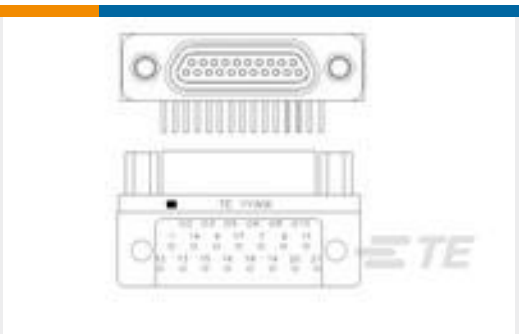
TE 产品编号1532260-4 M83513/13-C01NP = MCKS-N1-P-21SRT1
