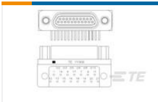
TE 产品编号1532260-2 M83513/13-C01CP = MCKS-C2-P-21SRT1
