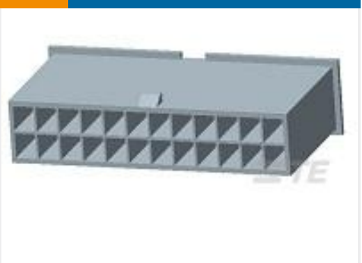
TE 产品编号2296206-4 4P FH PLUG VAL-U-LOK FH GWT/V0
