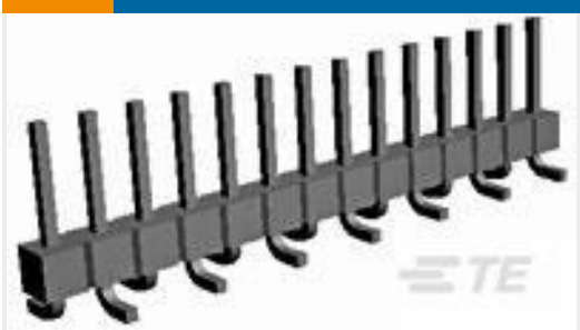
TE 产品编号1-640456-5 Polyester Vertical PCB Header: 2.54 mm, Unshrouded, No Mating Alignment
