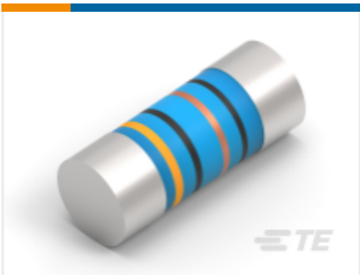
TE 产品编号2-2176315-3 MELF SMA_A 6K8 0.1% 15PPM 0204 0.4W
