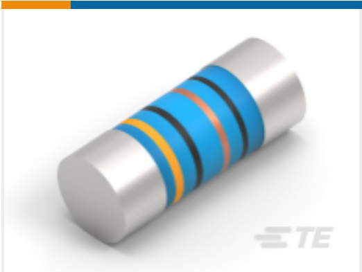
TE 产品编号2-2176315-3 MELF SMA_A 6K8 0.1% 15PPM 0204 0.4W
