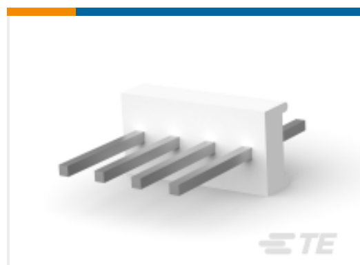
TE 产品编号1-640456-0 Polyester Vertical PCB Header: 2.54 mm, Unshrouded, No Mating Alignment
