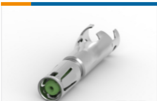
TE 产品编号2298116-1 MATE-AX, Socket outer contact, RTK 031
