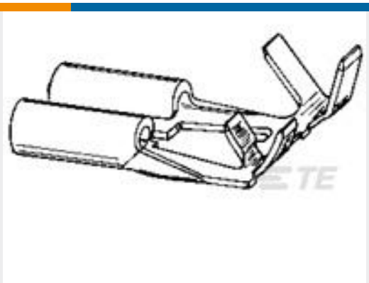
TE 产品编号160861-7 250 FASTON,FLAG,REC.,20-17 AWG, PB
