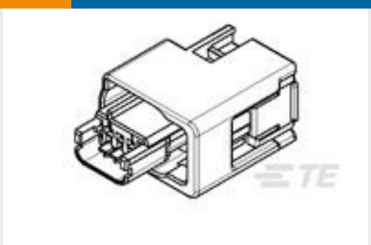
TE 产品编号1438454-1 0.64MM,3 POSN SEALED PLUG ASSY
