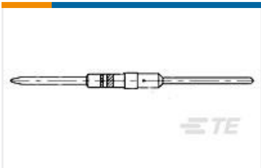
TE 产品编号448140-3 CONTACT,PIN,SZ 12,POSTED
