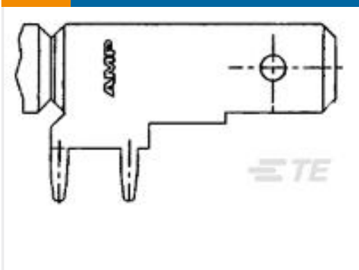
TE 产品编号1217754-1 250 FASTON, FLAG, PCB TAB, TNBR
