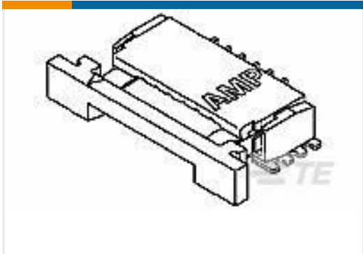
TE 产品编号2-84952-4 1MM FPC HORZ.BOTTOM CONT. ASSY 24P
