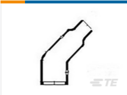
TE 产品编号467122-000 Heat Shrink Boots: Poly Mold, Lipped
