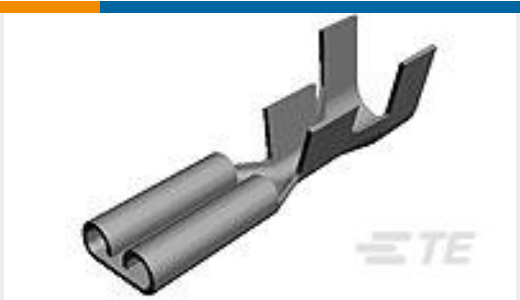
TE 产品编号41969-2 FASTON 250 TERMINAL REC 22-18 AWG BR
