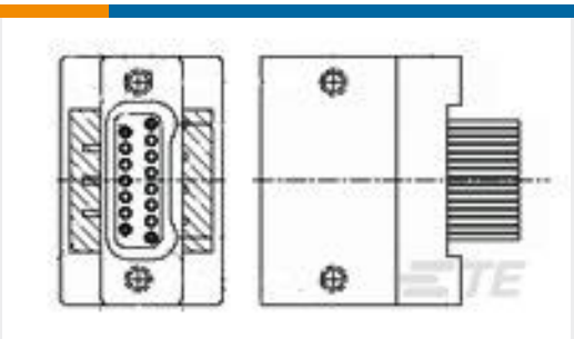
TE 产品编号1589488-7 STL009M5L = THRU-HOLE
