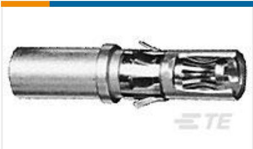
TE 产品编号193643-1 SKT ASSY.,POWER, #10-12 AWG
