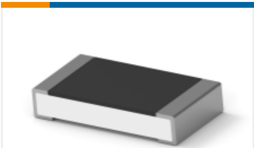
TE 产品编号2-2176389-9 RQ 1206 210R 0.1% 10PPM 5K RL
