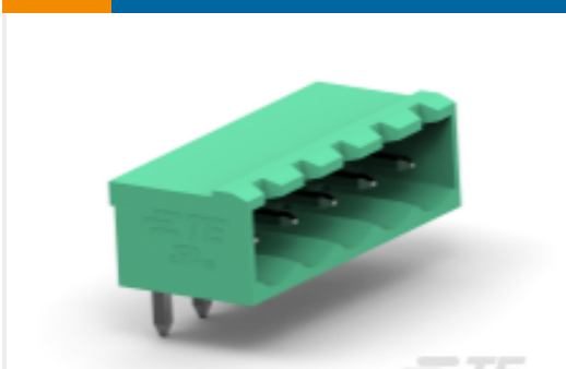
TE 产品编号1-2350513-2 12POS TB HDR 90 DEG, PITCH 5.0 &TL 4.5mm
