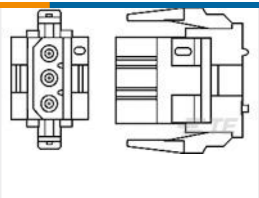
TE 产品编号1-640518-0 03P MR II PLUG HSG V0 RED
