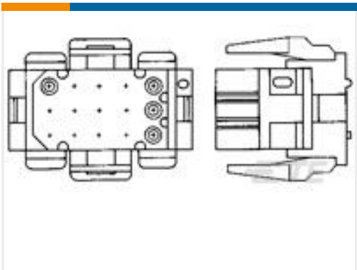
TE 产品编号1-640519-0 04P MR II PLUG HSG V0 RED
