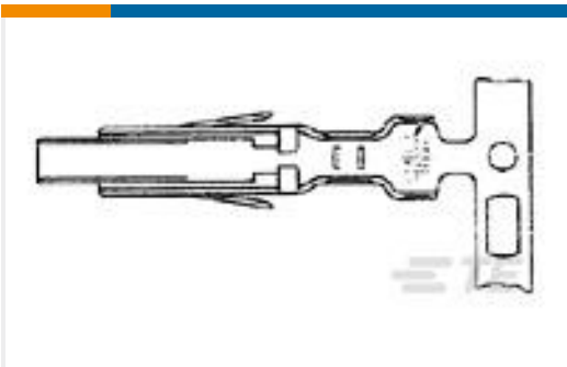
TE 产品编号170485-1 DRAWER CONN LP
