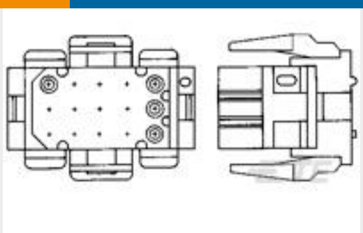
TE 产品编号1-640521-0 09P MR II PLUG HSG V0 RED
