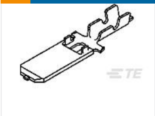
TE 产品编号170349-2 FF 250 TAB 22-20AWG TPBR WITHOUT LATCH
